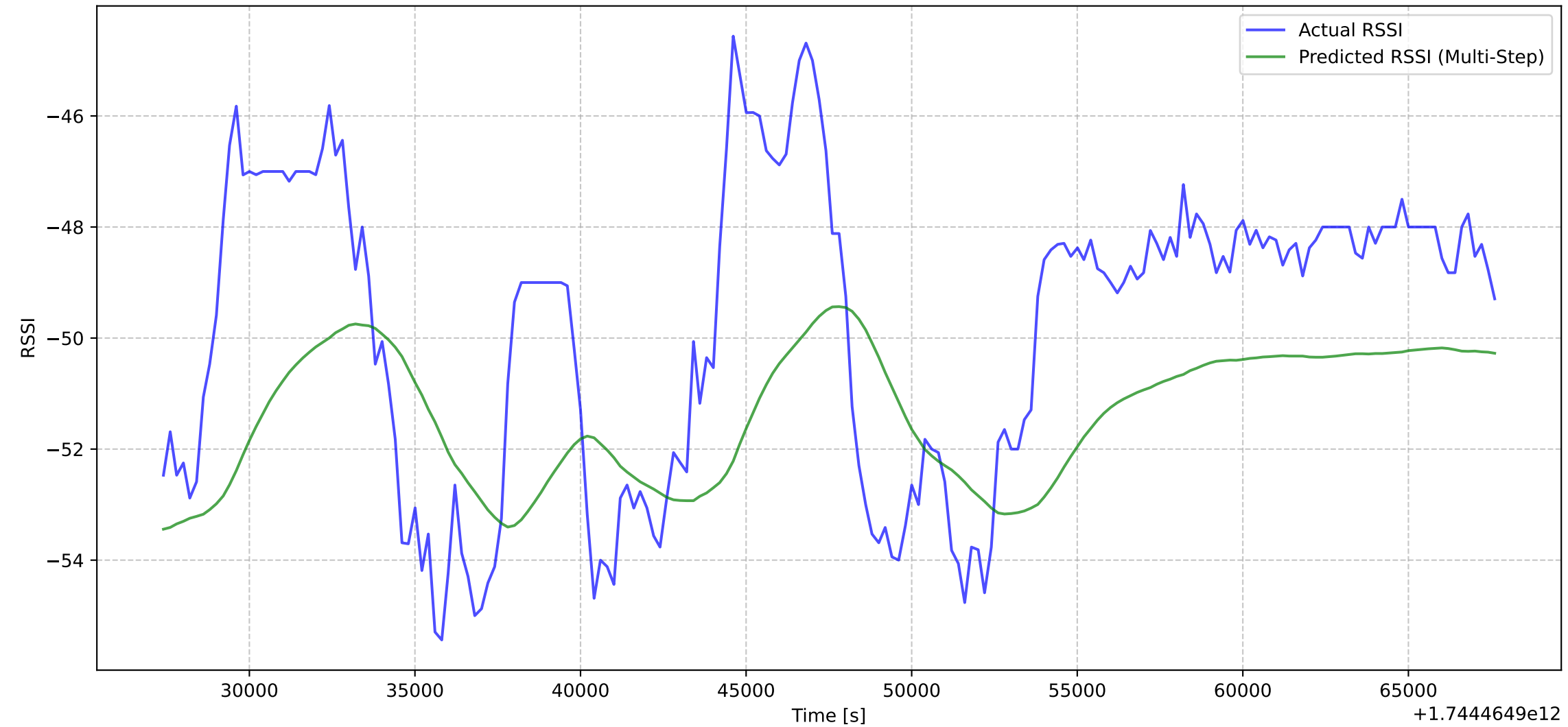
Actual vs Predicted RSSI (Multi-Step (step 20 \approx 4.0 s))
