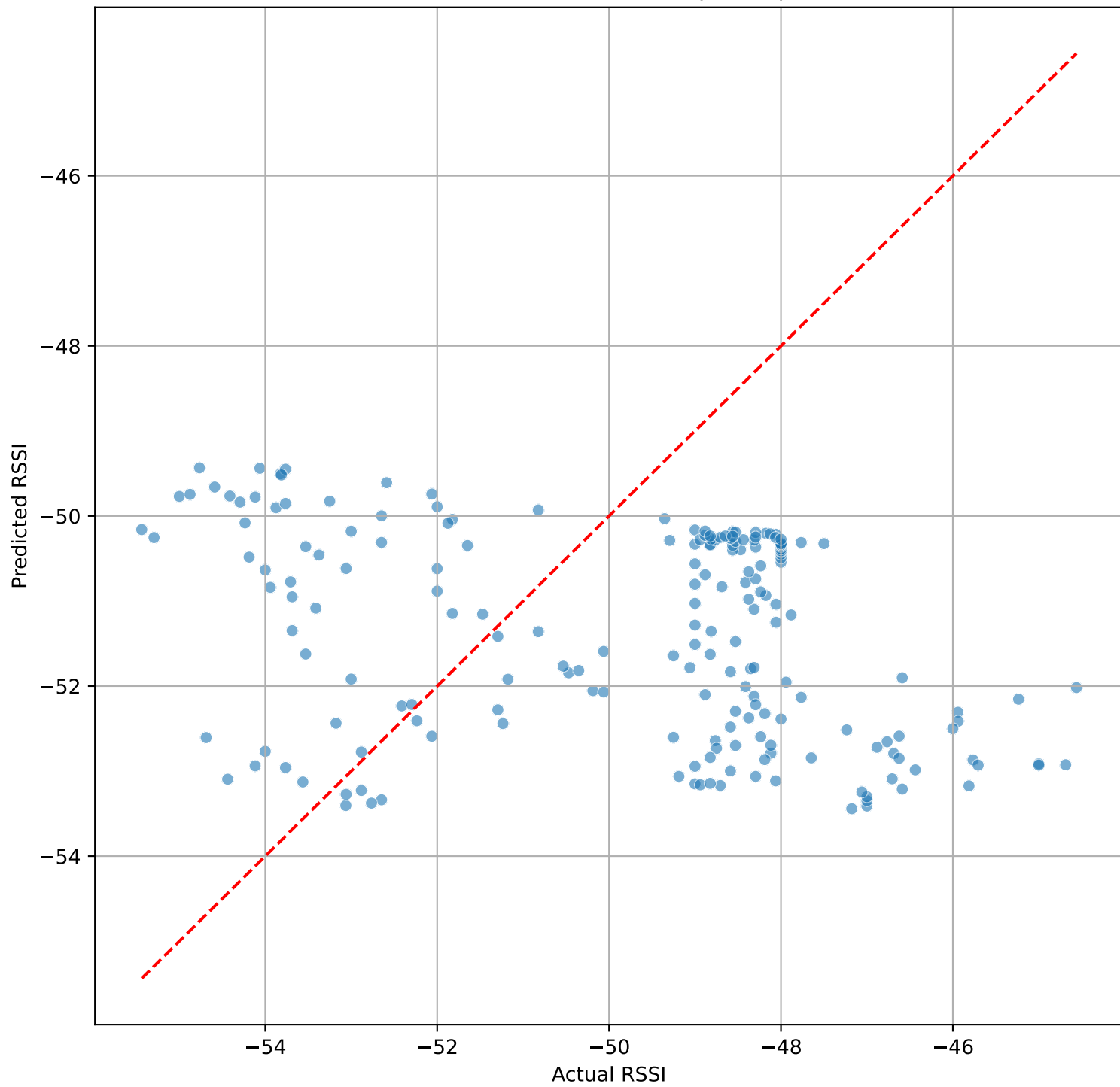
Actual vs Predicted RSSI (Last Step - step 20 \approx 4.0 s)
