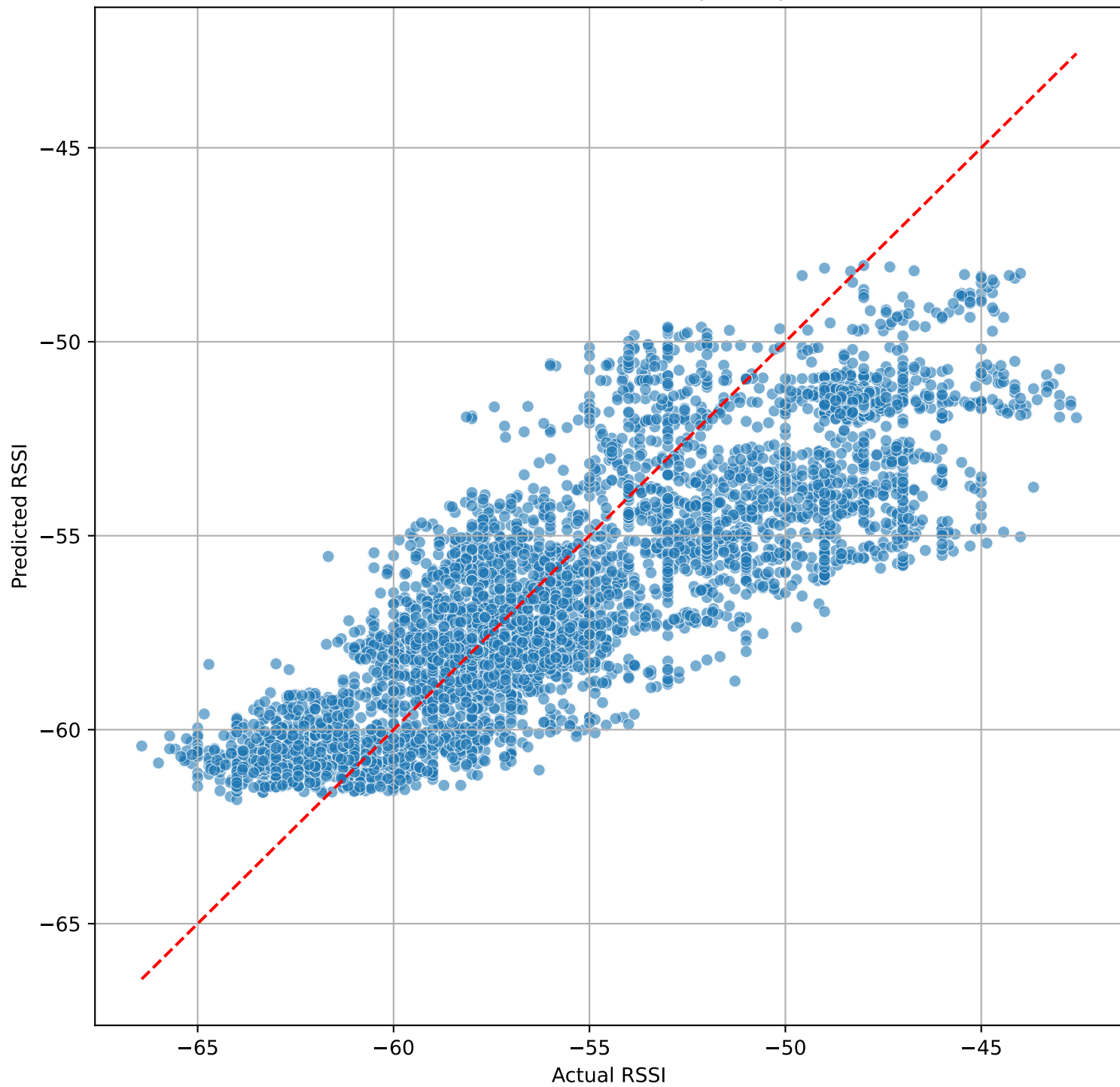
Actual vs Predicted RSSI (Last Step - step 40 \approx 4.0 s)
