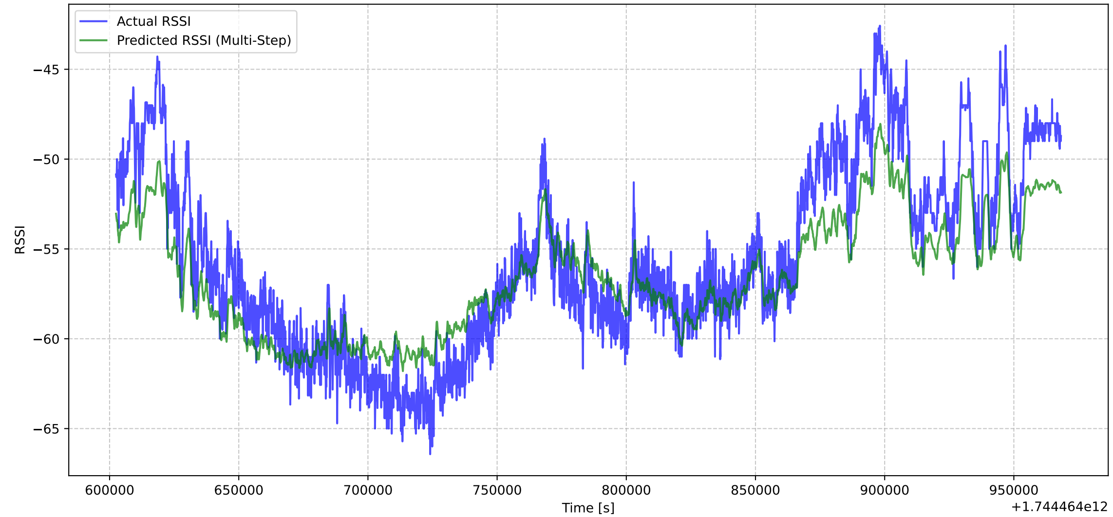
Actual vs Predicted RSSI (Multi-Step (step 40 \approx 4.0 s))
