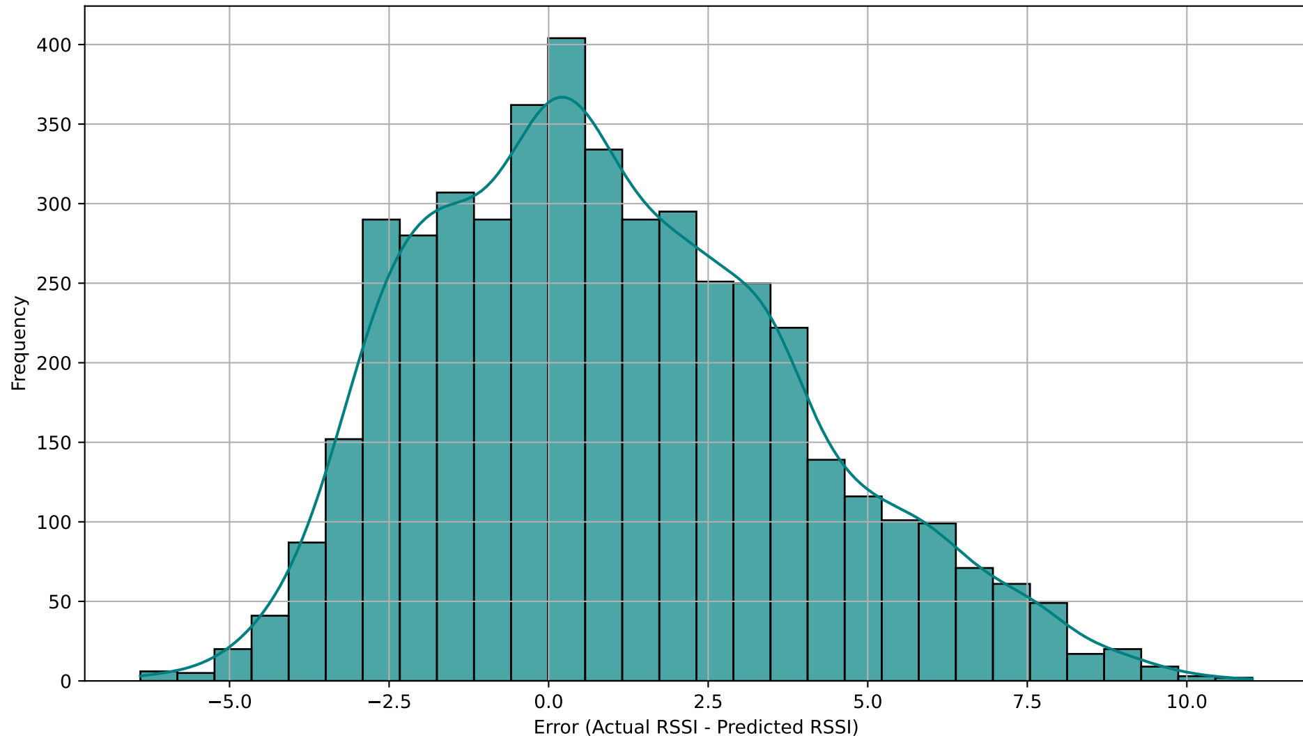
Distribution of Prediction Errors (Last Step - step 40 \approx 4.0 s)
