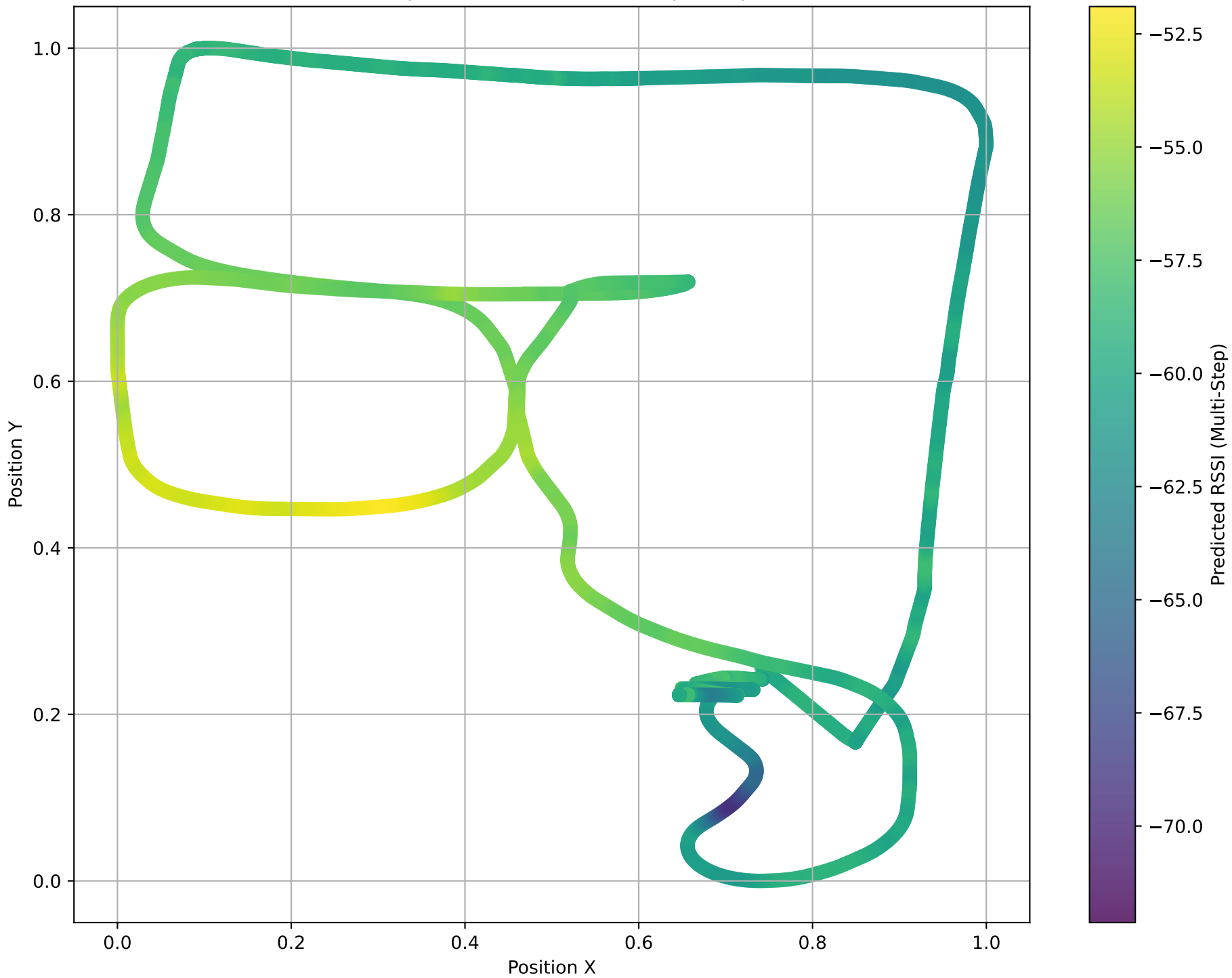
Predicted RSSI in Spatial Context (Multi-Step - step 120 \approx 10.0 s)
