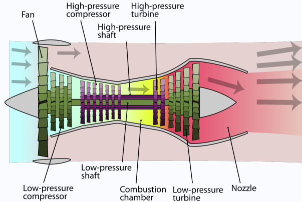
Figure: Major components of turbofans
