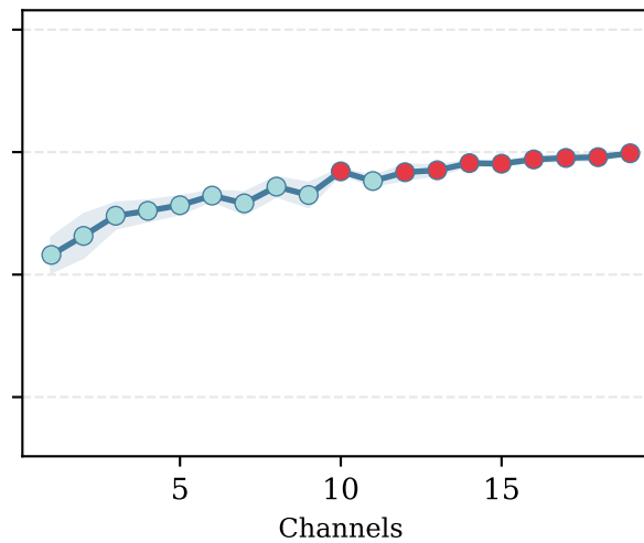
Georgia (F1)
