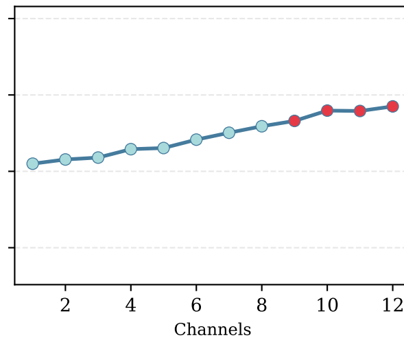
CPSC (F1)
