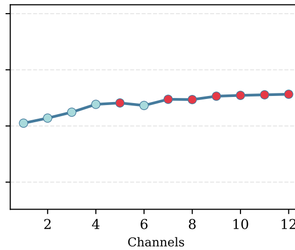
Georgia (F1)
