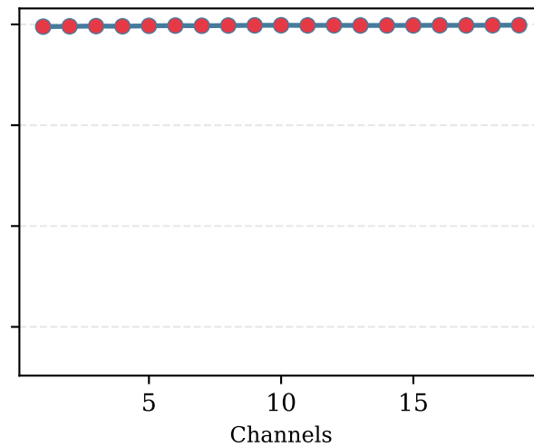
CPSC (F1)
