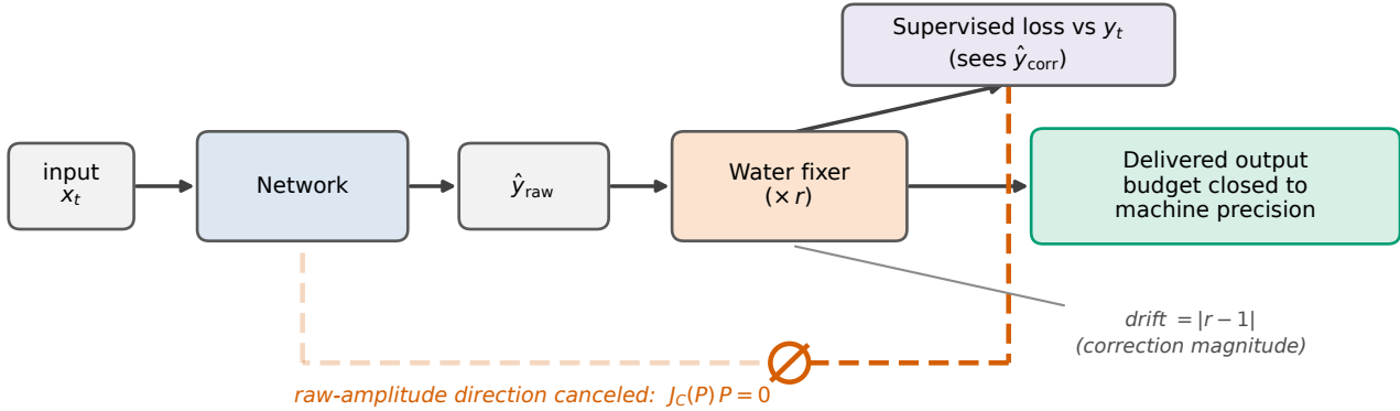
(b) Hard corrector inside the loss — scale degeneracy
