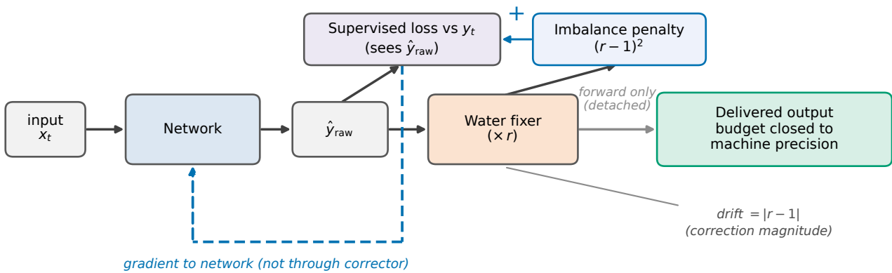
(c) Decoupled loss + imbalance penalty
