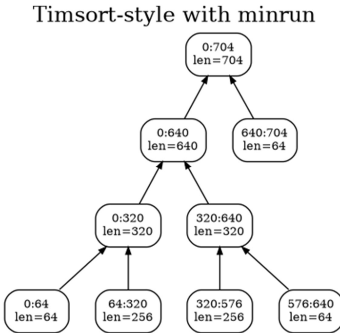
Figure 4(a). Timsort-style merge tree for the illustrative run sequence.
