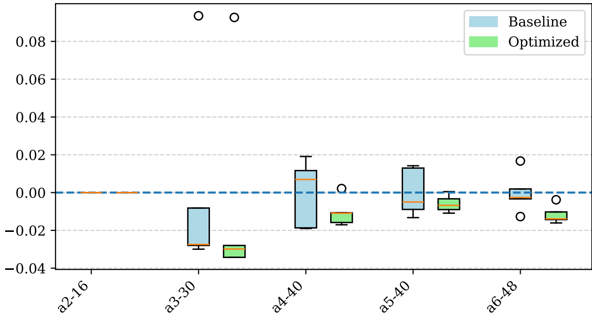
Relative gap (objective value)
