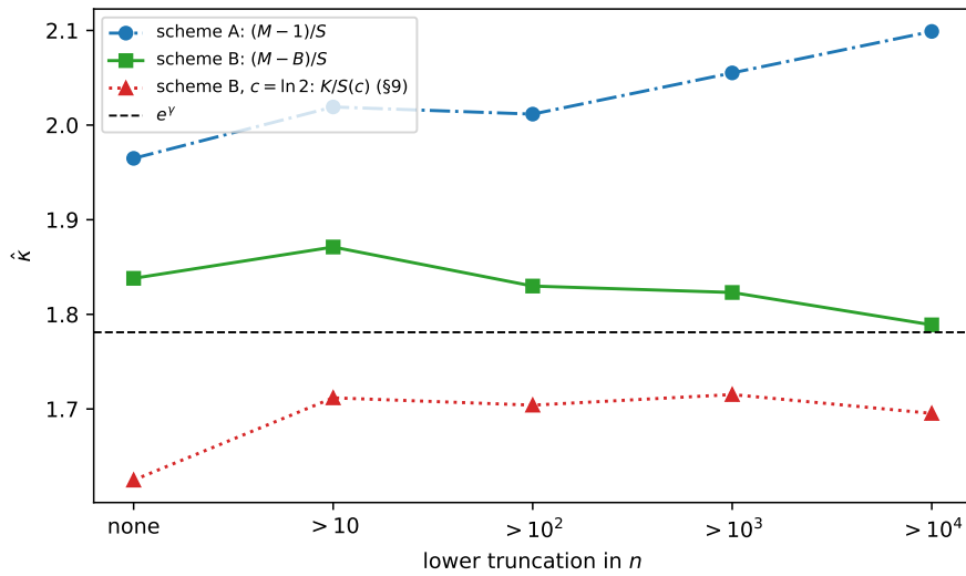
Figure 2. The pooled estimate under lower truncation: (M - 1)/S (scheme A), (M - B)/S (scheme B) and K/S(c) with the second-order term c = \ln 2 (§9). The upward trend of scheme A disappears under scheme B; the residual decline of scheme B disappears once the second-order term is included.
