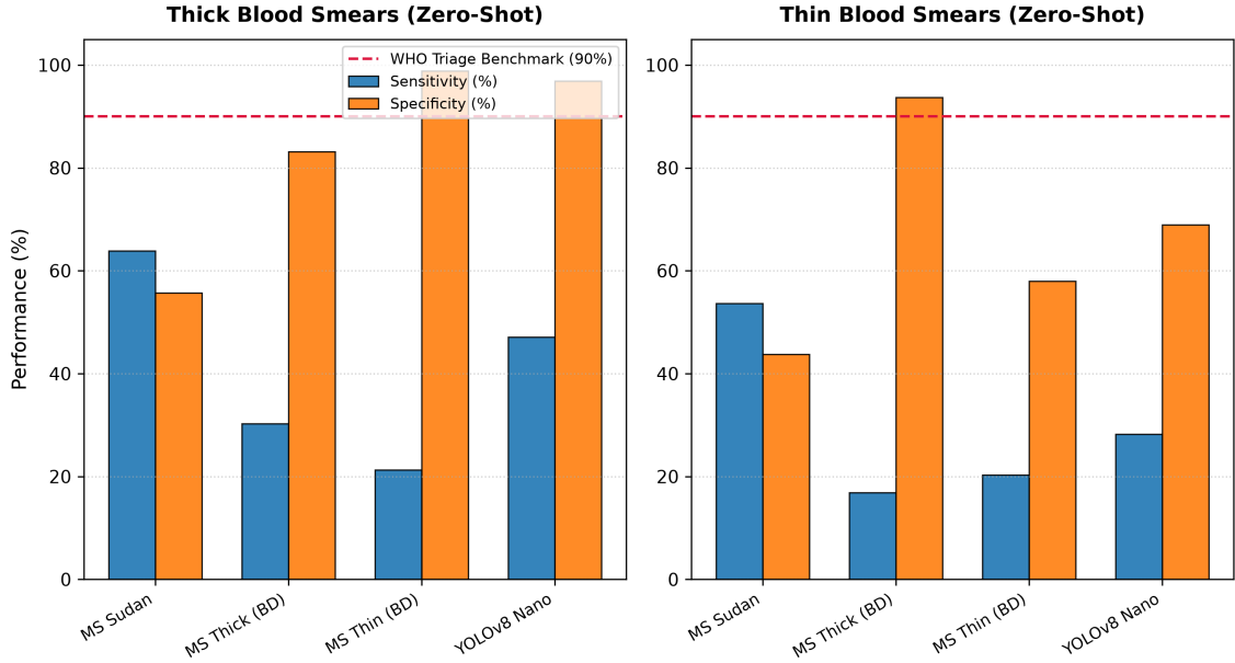
Figure 2: Comparative diagnostic sensitivity and specificity across thick ( N = 3,902 ) and thin ( N = 2,555 ) blood smears under zero-shot transfer. The dashed red line denotes the WHO Level-1 screening requirement ( \geq 90\% ). Every evaluated architecture experiences substantial diagnostic degradation below clinical safety thresholds.
