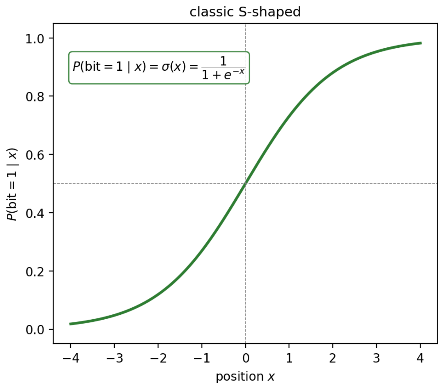
activated transfer function
