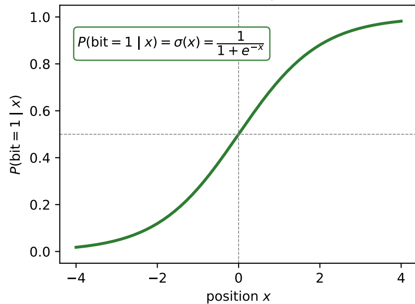
classic S-shaped
