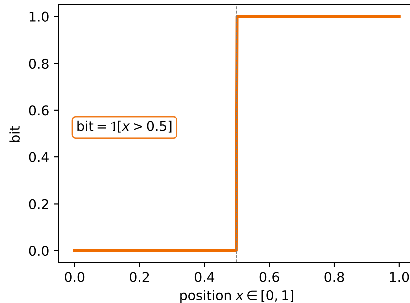
hard threshold
