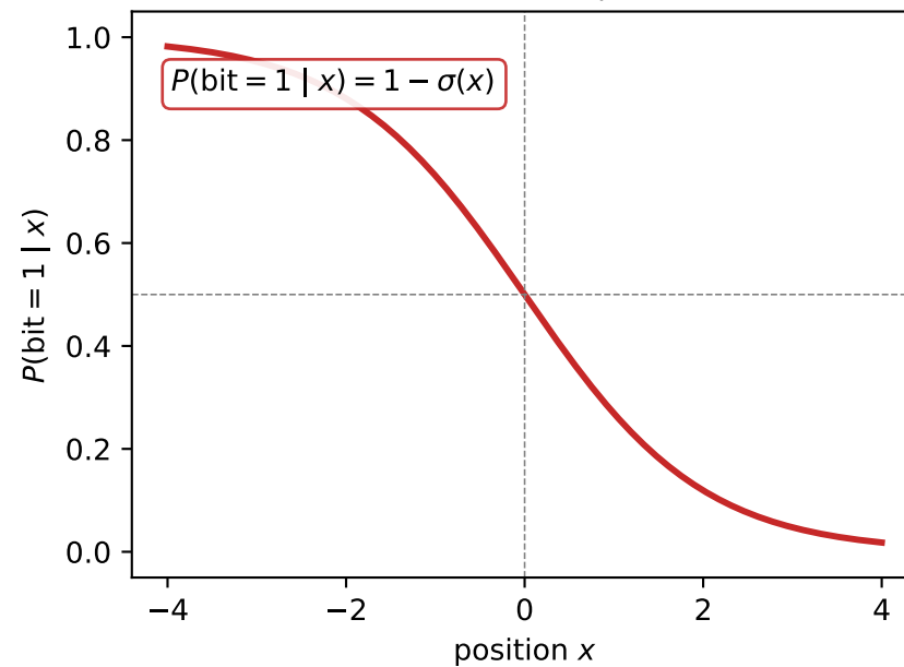
second S-shaped
