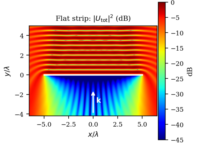
Fig. 1. Flat strip ( A = 0 , L = 10\lambda , N = 200 ): normalized total near-field intensity |U_{\text{tot}}|^2 in dB. The arrow marks the incident-wave direction.
