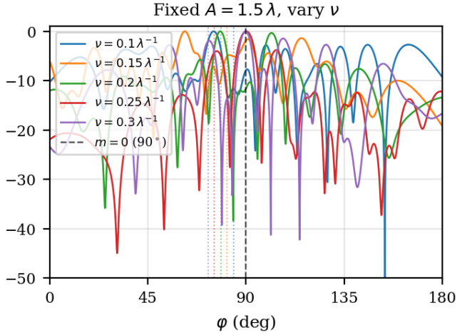
Fig. 6. Forward-hemisphere pattern evolution at fixed A = 1.5\lambda as \nu varies. Dotted verticals mark the m = +1 reference angle for each spatial frequency.
