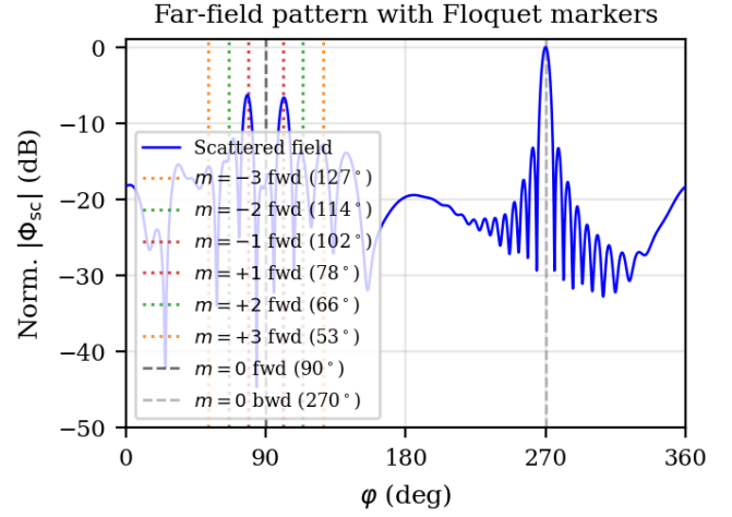
Fig. 4. Sinusoidal strip normalized scattered far-field amplitude. Vertical markers show infinite-periodic Floquet reference angles.
