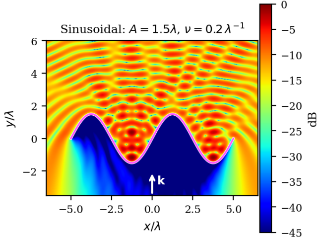
Fig. 3. Sinusoidal strip ( A = 1.5\lambda , \nu = 0.20 \lambda^{-1} ): normalized total near-field intensity with the strip profile overlaid.
