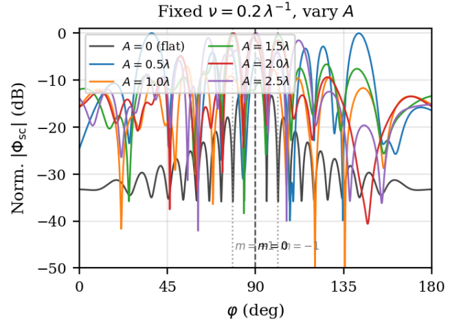
Fig. 5. Forward-hemisphere pattern evolution at fixed \nu = 0.20 \lambda^{-1} as A varies. Dotted verticals mark the m = \pm 1 Floquet-reference angles.
