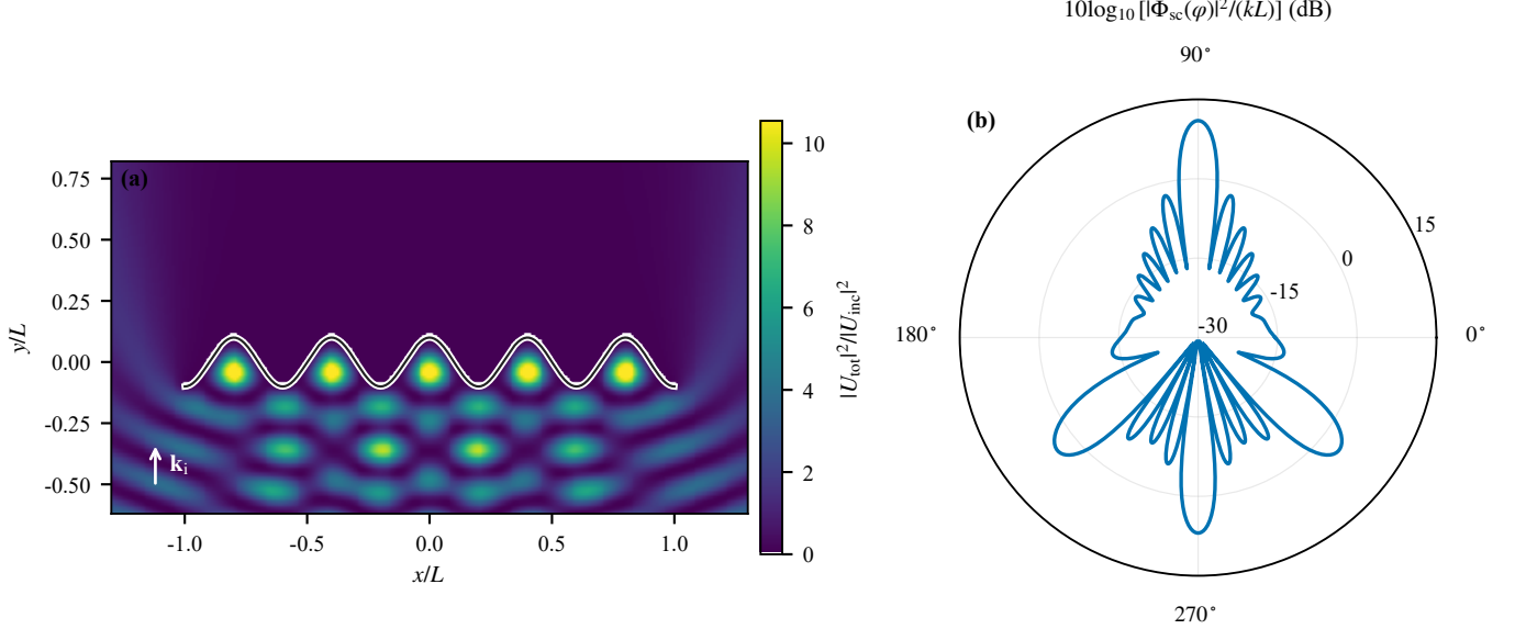
Fig. 3. Five-period grating at P = 5 , h/L = 0.10 , kL = 20 , and \beta = \pi/2 . (a) Relative total-field intensity |U^{\text{inc}} + U^{\text{sc}}|^2 / |U^{\text{inc}}|^2 . (b) Absolute polar scattering diagram based on \Phi_{\text{sc}} in (15), shown as 10 \log_{10}[|\Phi_{\text{sc}}(\varphi)|^2 / (kL)] on the common -30 to +15 dB scale.
