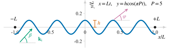
Fig. 1. Symmetric finite sinusoidal PEC grating and angle convention. The pale coordinate axes at x = 0 and y = 0 are the symmetry axis and mean line; the tick-ended orange segment denotes the corrugation height h . The incident wave vector is \mathbf{k}_i = k\mathbf{d} , where \mathbf{d} = (\cos \beta, \sin \beta) ; observation angle \varphi is measured counterclockwise from +x .
