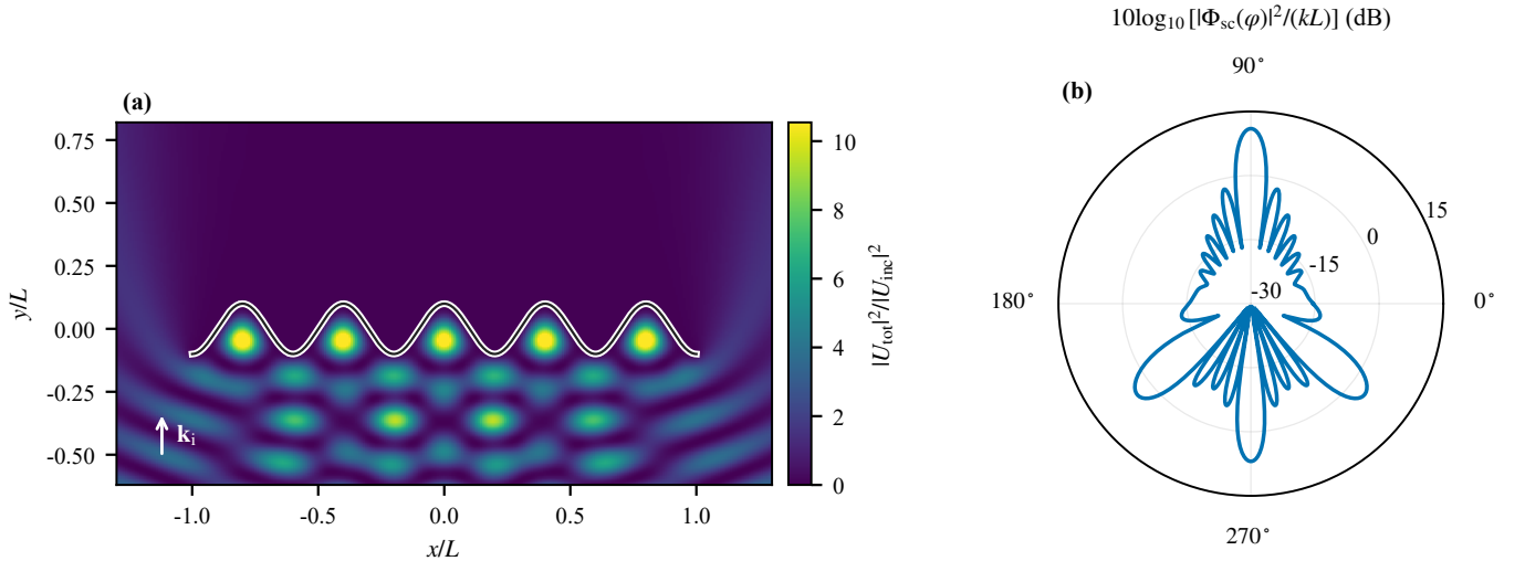
Fig. 3. Five-period grating at P = 5 , h/L = 0.10 , kL = 20 , and \beta = \pi/2 . (a) Relative total-field intensity |U^{\text{inc}} + U^{\text{sc}}|^2 / |U^{\text{inc}}|^2 . (b) Absolute polar scattering diagram based on \Phi_{\text{sc}} in (15), shown as 10 \log_{10}[|\Phi_{\text{sc}}(\varphi)|^2 / (kL)] on the common -30 to +15 dB scale.
