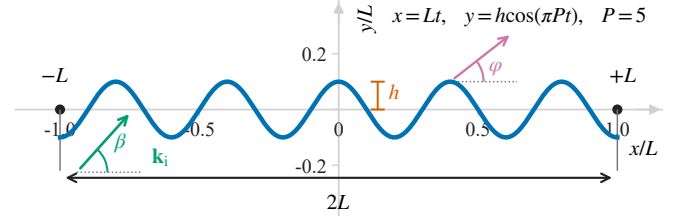
Fig. 1. Symmetric finite sinusoidal PEC grating and angle convention. The pale coordinate axes at x = 0 and y = 0 are the symmetry axis and mean line; the tick-ended orange segment denotes the corrugation height h . The incident wave vector is \mathbf{k}_i = k\hat{\mathbf{d}} , where \hat{\mathbf{d}} = (\cos \beta, \sin \beta) ; observation angle \varphi is measured counterclockwise from +x .
