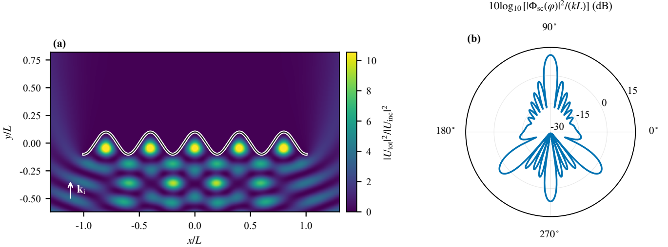
Fig. 3. Five-period grating at P = 5 , h/L = 0.10 , kL = 20 , and \beta = \pi/2 . (a) Relative total-field intensity |U_{\text{inc}} + U^{\text{sc}}|^2/|U_{\text{inc}}|^2 . (b) Absolute polar scattering diagram based on \Phi_{\text{sc}} in (15), shown as 10 \log_{10} [|\Phi_{\text{sc}}(\varphi)|^2/(kL)] on the common -30 to +15 dB scale.
