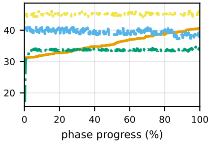
concurrency 1
