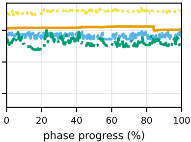
concurrency 16
