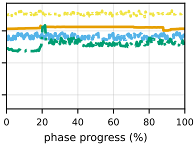
concurrency 8
