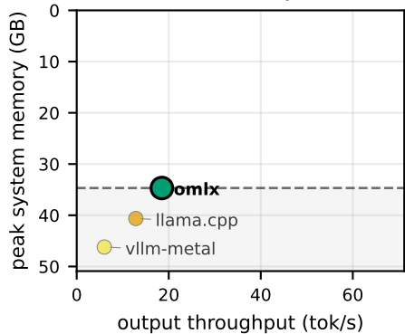
concurrency 1
