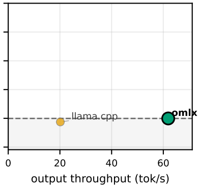
concurrency 16
