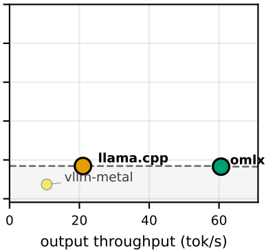
concurrency 8
