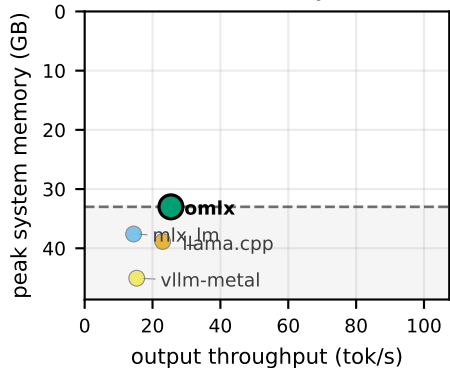
concurrency 1
