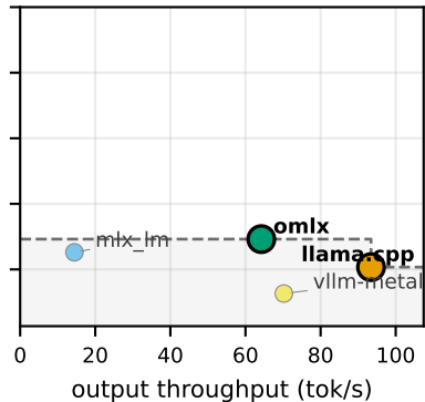
concurrency 16
