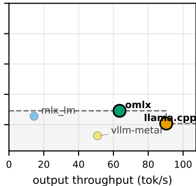
concurrency 8
