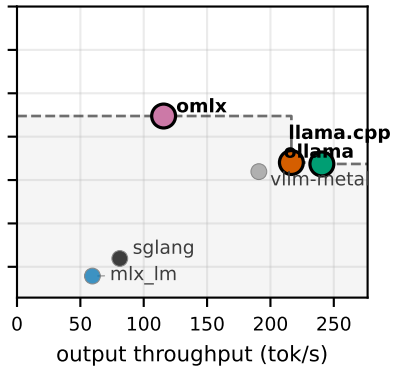
concurrency 16
