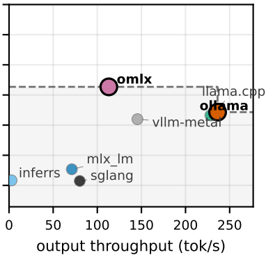
concurrency 8
