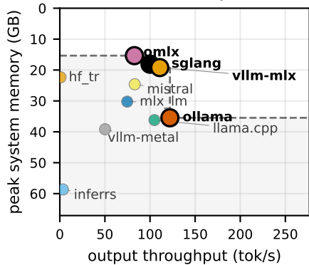
concurrency 1
