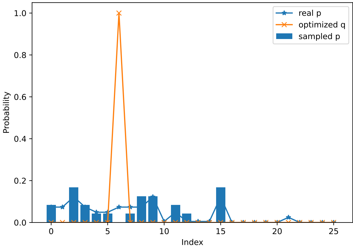
Target vs optimized distribution (alpha=1.0)
