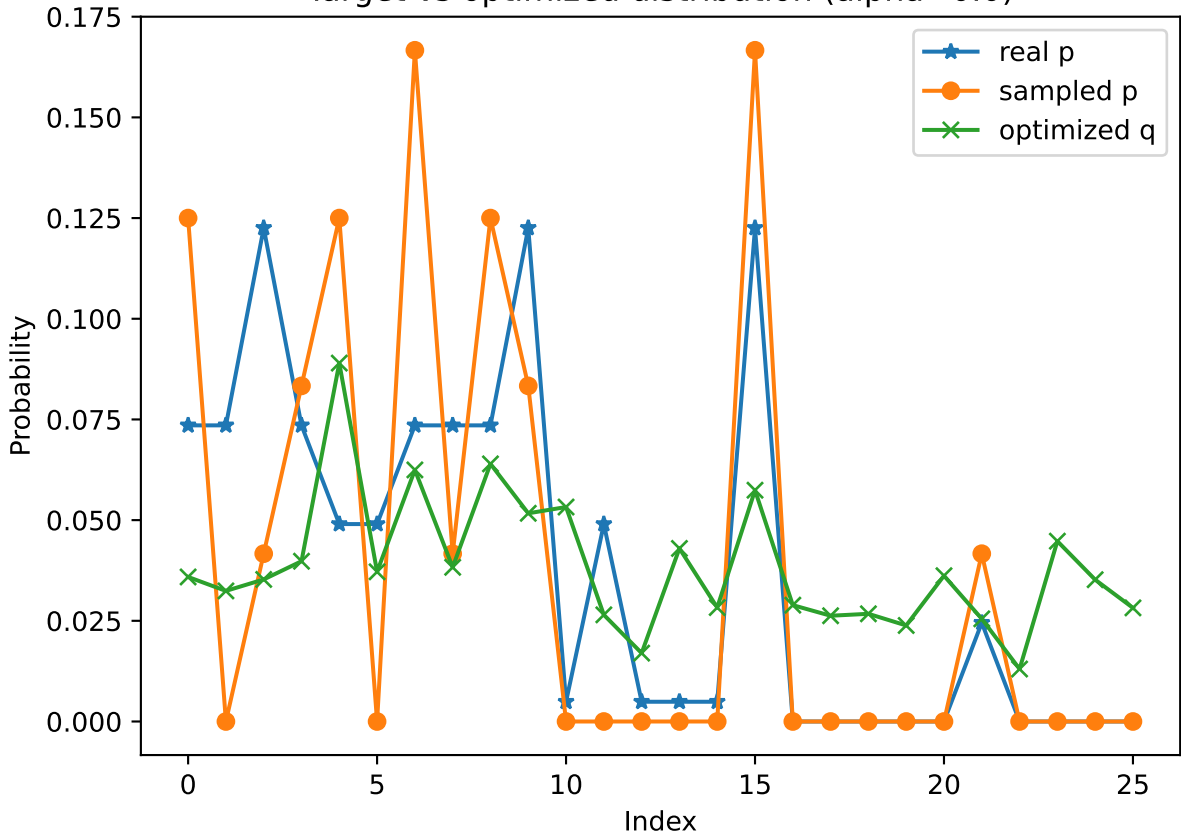
Target vs optimized distribution (alpha=0.0)
