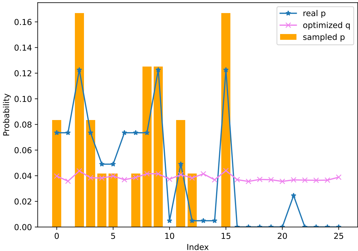
Target vs optimized distribution (alpha=0.99)
