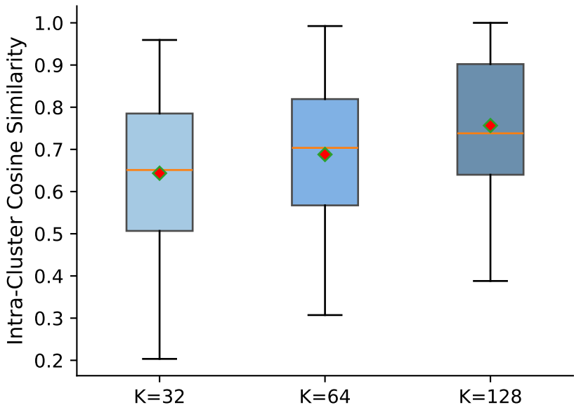
Semantic Coherence by Cluster Granularity
