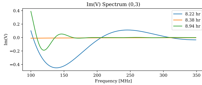
Figure 37: Imaginary visibility vs frequency for baseline (0,3).
