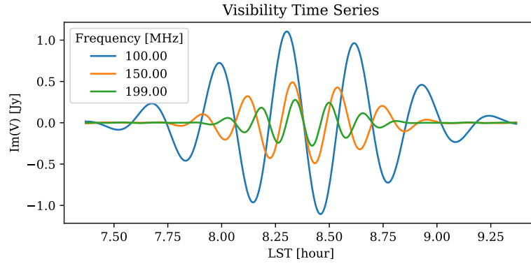
Figure 7: Imaginary visibility vs LST.
