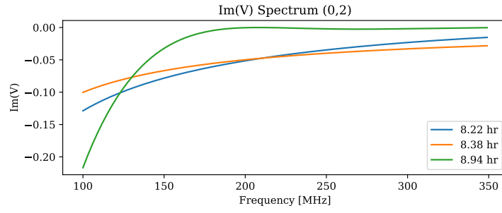
Figure 36: Imaginary visibility vs frequency for baseline (0,2).
