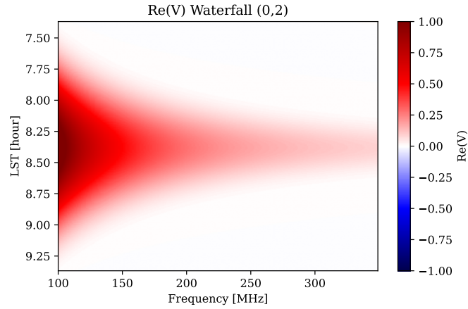
Figure 42: Real visibility waterfall for baseline (0,2).
