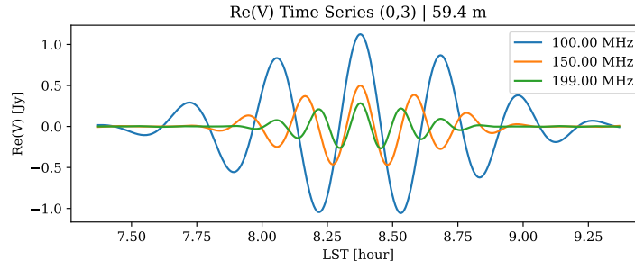
Figure 19: Real visibility vs LST for baseline (0,3).
