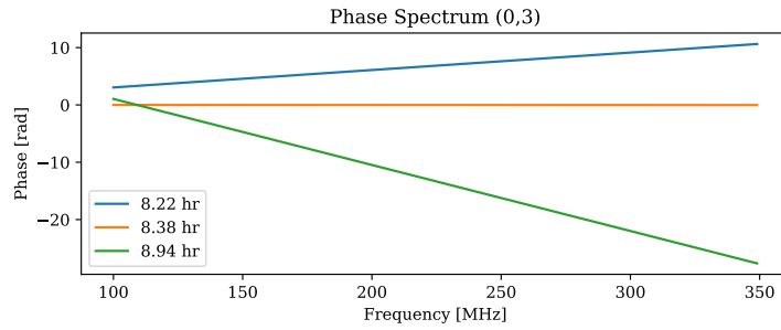
Figure 40: Visibility phase vs frequency for baseline (0,3).
