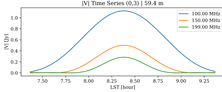
Figure 22: Visibility amplitude vs LST for baseline (0,3).
