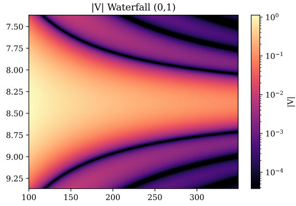
Figure 44: Amplitude waterfall for baseline (0,1).
