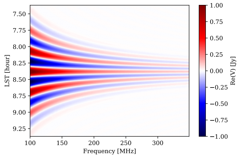
Figure 13: Real part waterfall.
