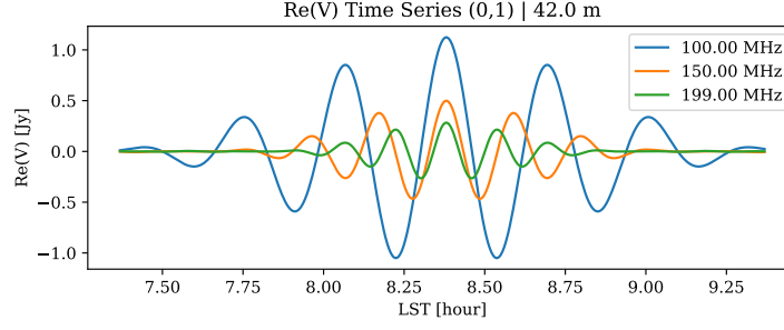
Figure 17: Real visibility vs LST for baseline (0,1).
