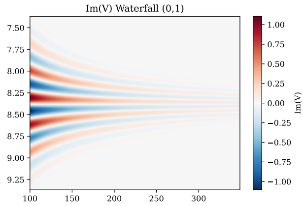
Figure 47: Imaginary visibility waterfall for baseline (0,1).
