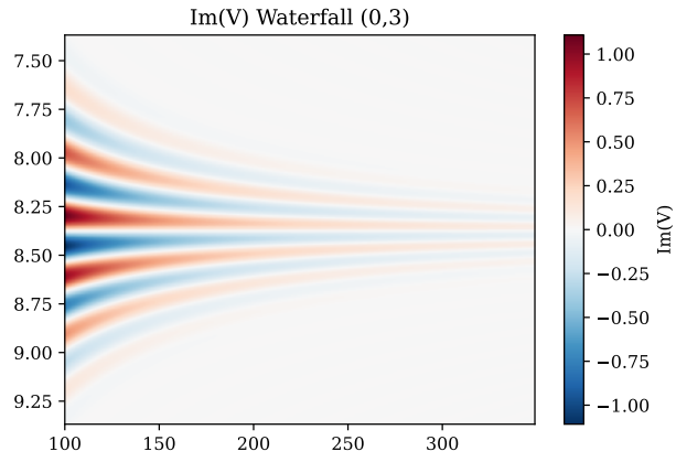
Figure 49: Imaginary visibility waterfall for baseline (0,3).
