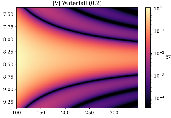
Figure 45: Amplitude waterfall for baseline (0,2).
