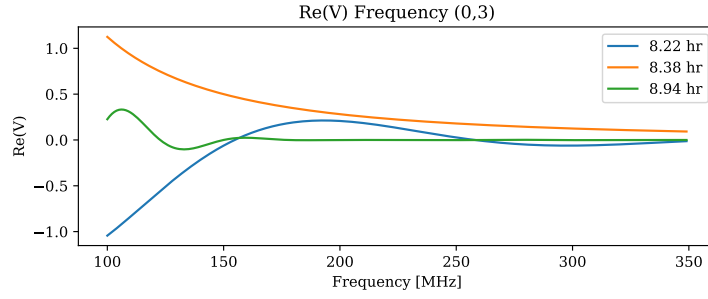
Figure 31: Real visibility vs frequency for baseline (0,3).
