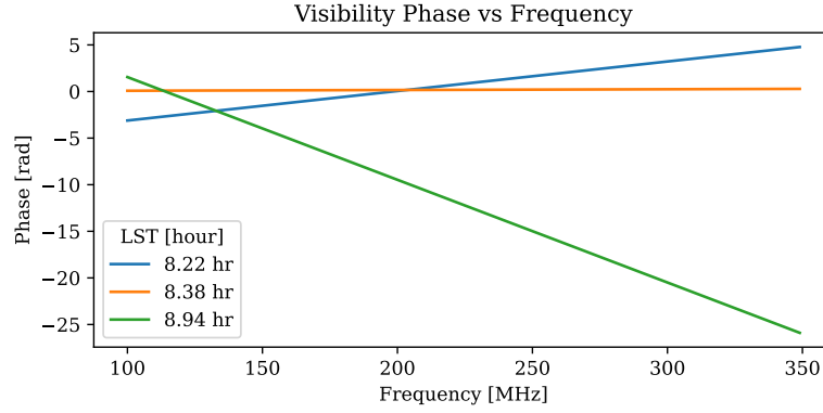
Figure 11: Unwrapped visibility phase as a function of frequency for selected LST values. The approximately linear dependence reflects the geometric delay term in the measurement equation.
