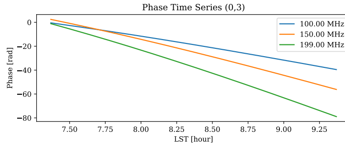
Figure 28: Visibility phase vs LST for baseline (0,3).
