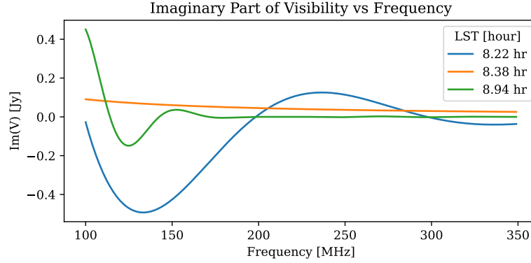
Figure 10: Imaginary part of the visibility as a function of frequency for selected LST values. Oscillations arise from the frequency-dependent interferometric fringe term.
