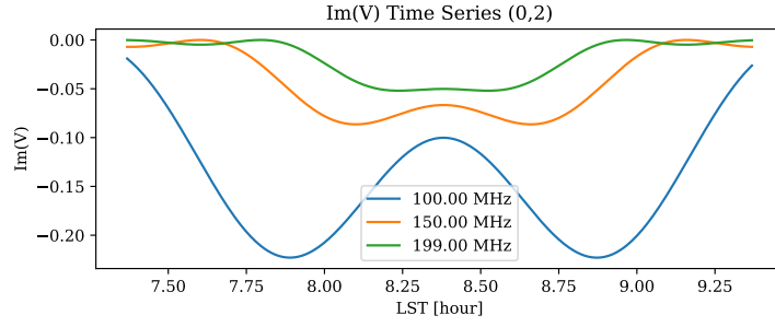
Figure 24: Imaginary visibility vs LST for baseline (0,2).
