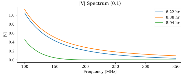
Figure 32: Visibility amplitude vs frequency for baseline (0,1).
