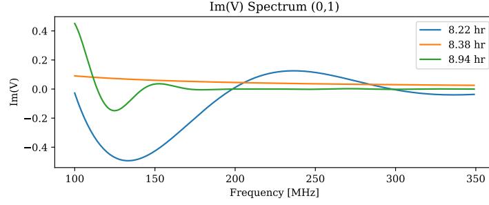
Figure 35: Imaginary visibility vs frequency for baseline (0,1).
