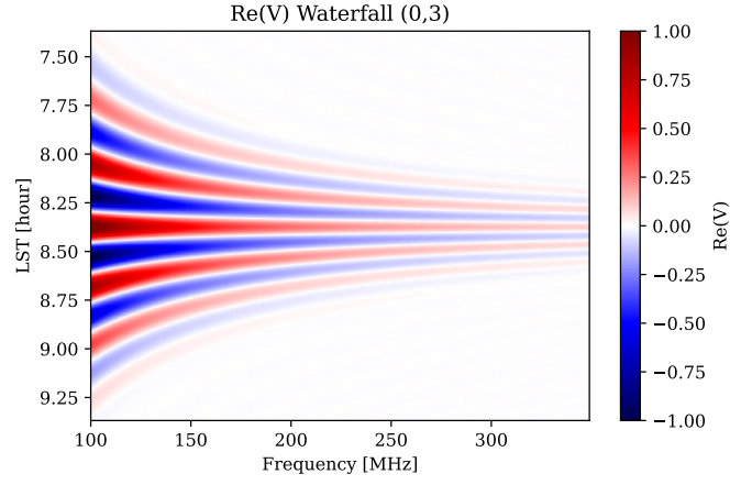
Figure 43: Real visibility waterfall for baseline (0,3).
