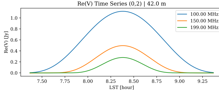
Figure 18: Real visibility vs LST for baseline (0,2).
