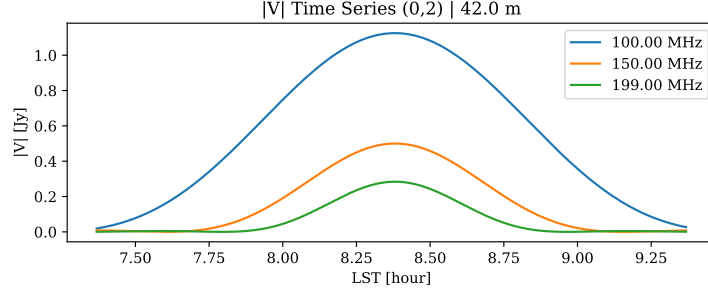
Figure 21: Visibility amplitude vs LST for baseline (0,2).
