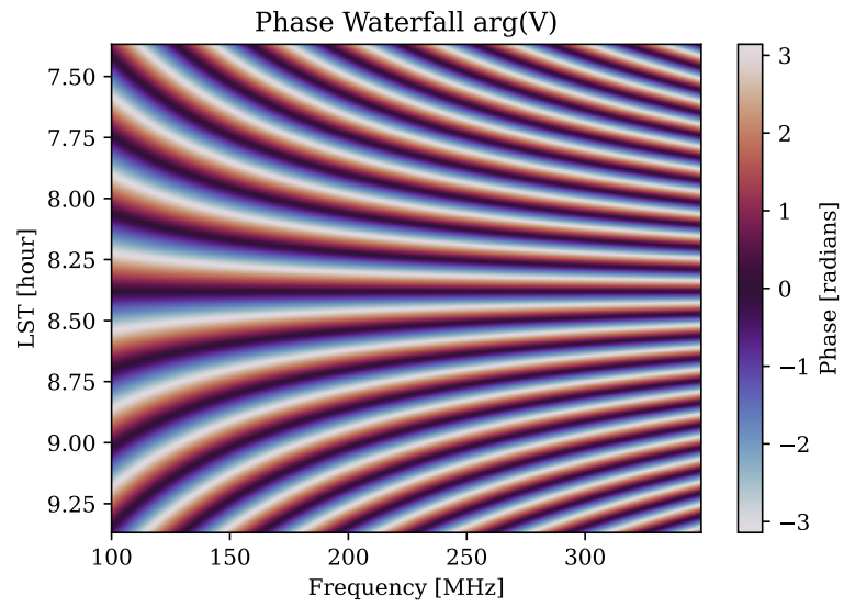
Figure 16: Phase waterfall.
