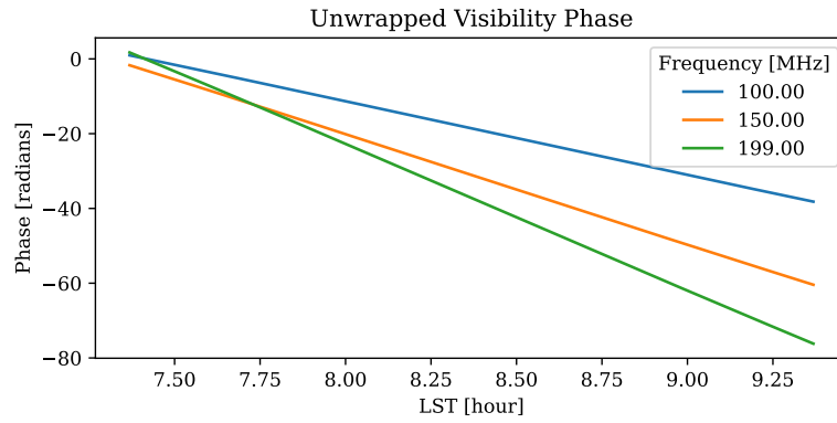
Figure 8: Phase evolution of visibility.
