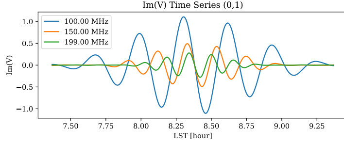
Figure 23: Imaginary visibility vs LST for baseline (0,1).
