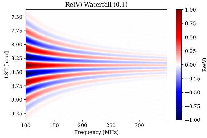
Figure 41: Real visibility waterfall for baseline (0,1).
