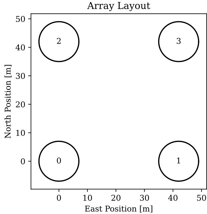
Figure 4: Array layout of the interferometric telescope. Each antenna position defines a baseline pair, which measures complex visibilities sensitive to sky brightness distributions.
