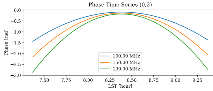
Figure 27: Visibility phase vs LST for baseline (0,2).
