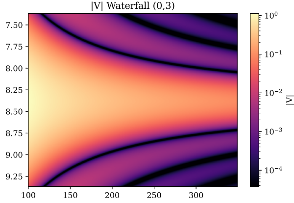
Figure 46: Amplitude waterfall for baseline (0,3).
