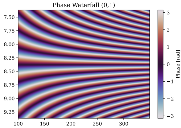
Figure 50: Phase waterfall for baseline (0,1).
