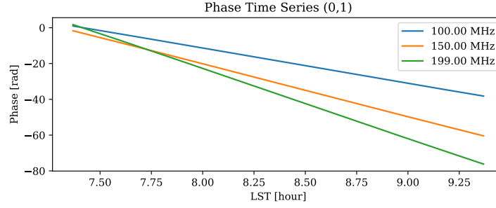
Figure 26: Visibility phase vs LST for baseline (0,1).
