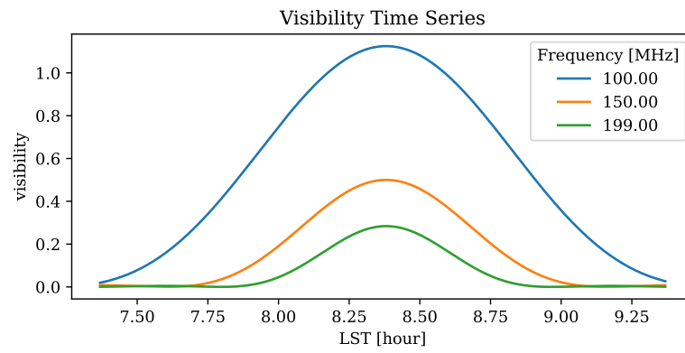
Figure 6: Visibility amplitude vs LST.
