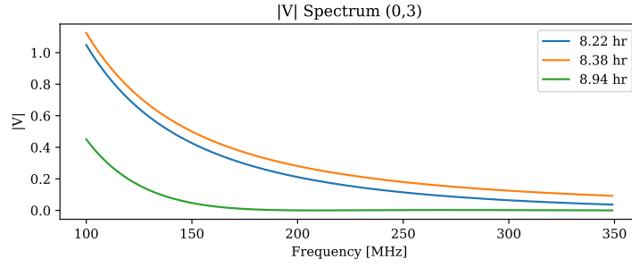
Figure 34: Visibility amplitude vs frequency for baseline (0,3).
