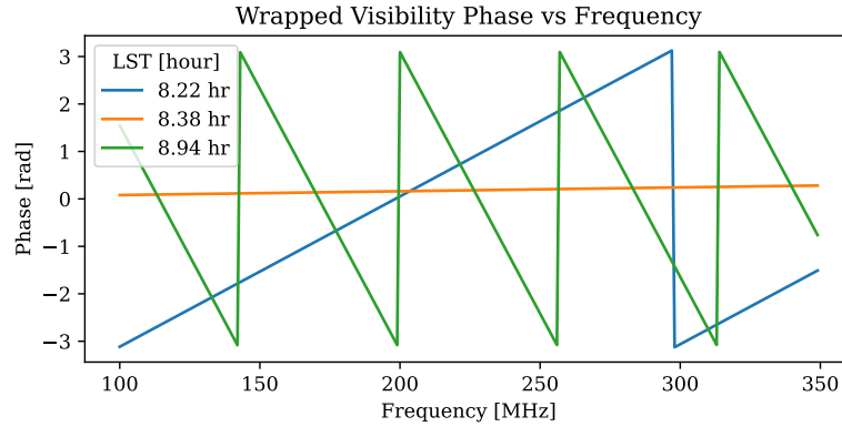
Figure 12: wrapped visibility phase as a function of frequency for selected LST values. The approximately linear dependence reflects the geometric delay term in the measurement equation.
