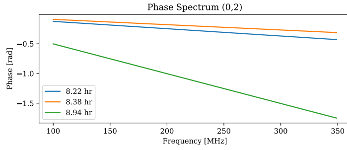
Figure 39: Visibility phase vs frequency for baseline (0,2).
