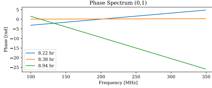
Figure 38: Visibility phase vs frequency for baseline (0,1).
