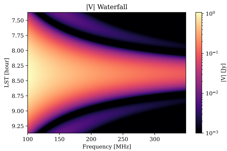
Figure 14: Amplitude waterfall.
