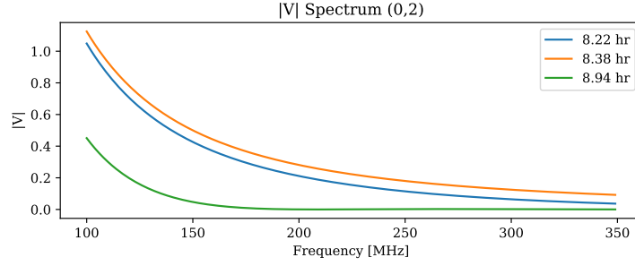
Figure 33: Visibility amplitude vs frequency for baseline (0,2).
