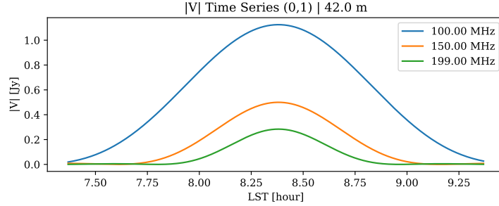
Figure 20: Visibility amplitude vs LST for baseline (0,1).
