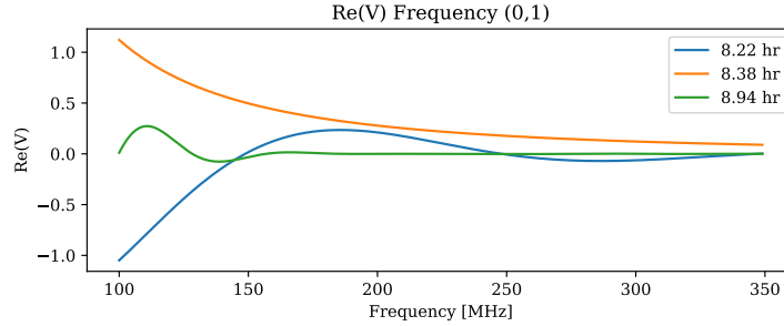
Figure 29: Real visibility vs frequency for baseline (0,1).
