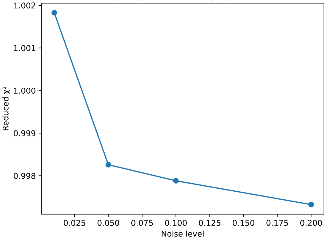
Fit quality vs noise (2D polynomial)
