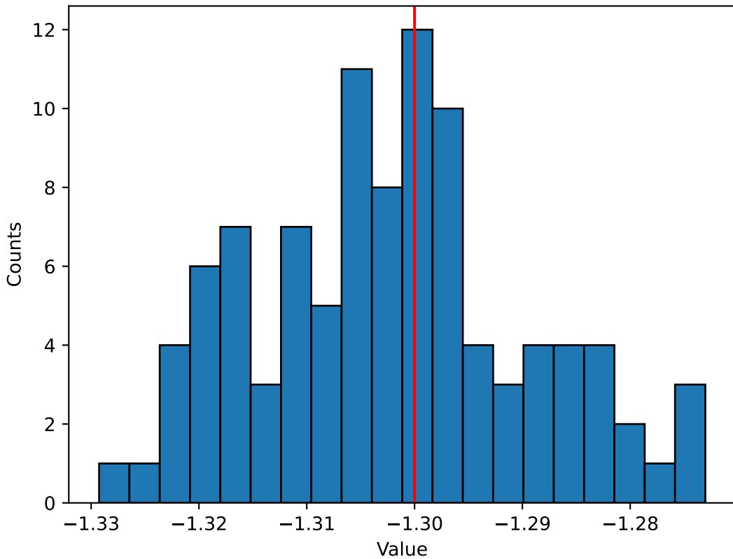
Coefficient 0 distribution
