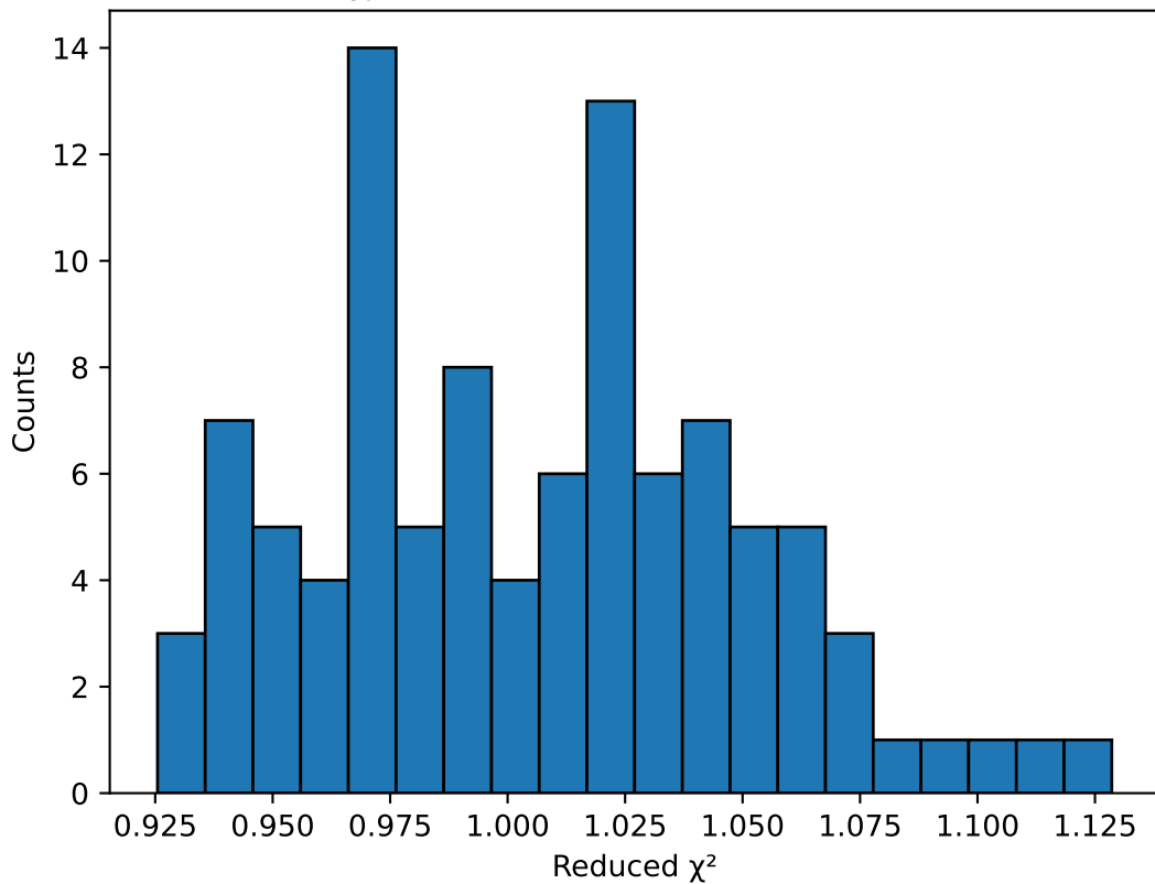
Sine \chi^2 distribution over noise realizations
