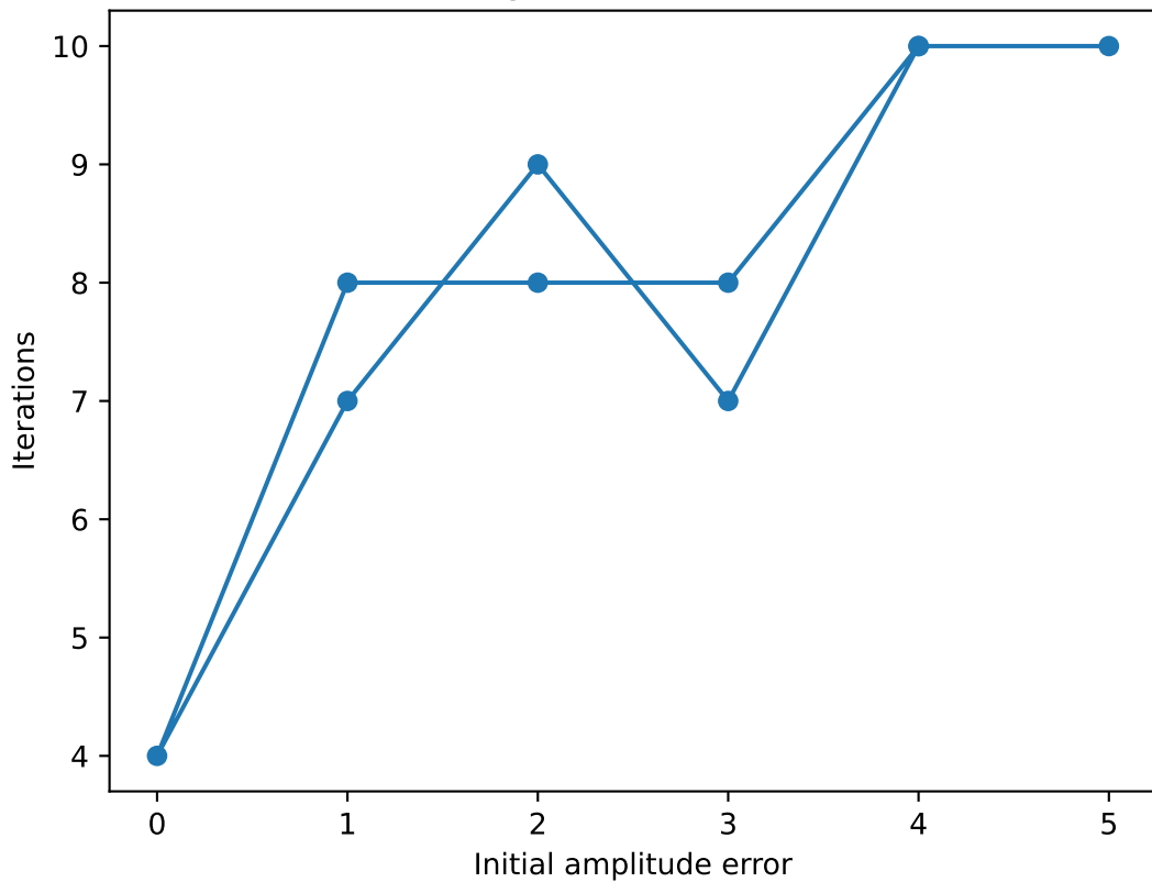
Convergence vs Initial Guess
