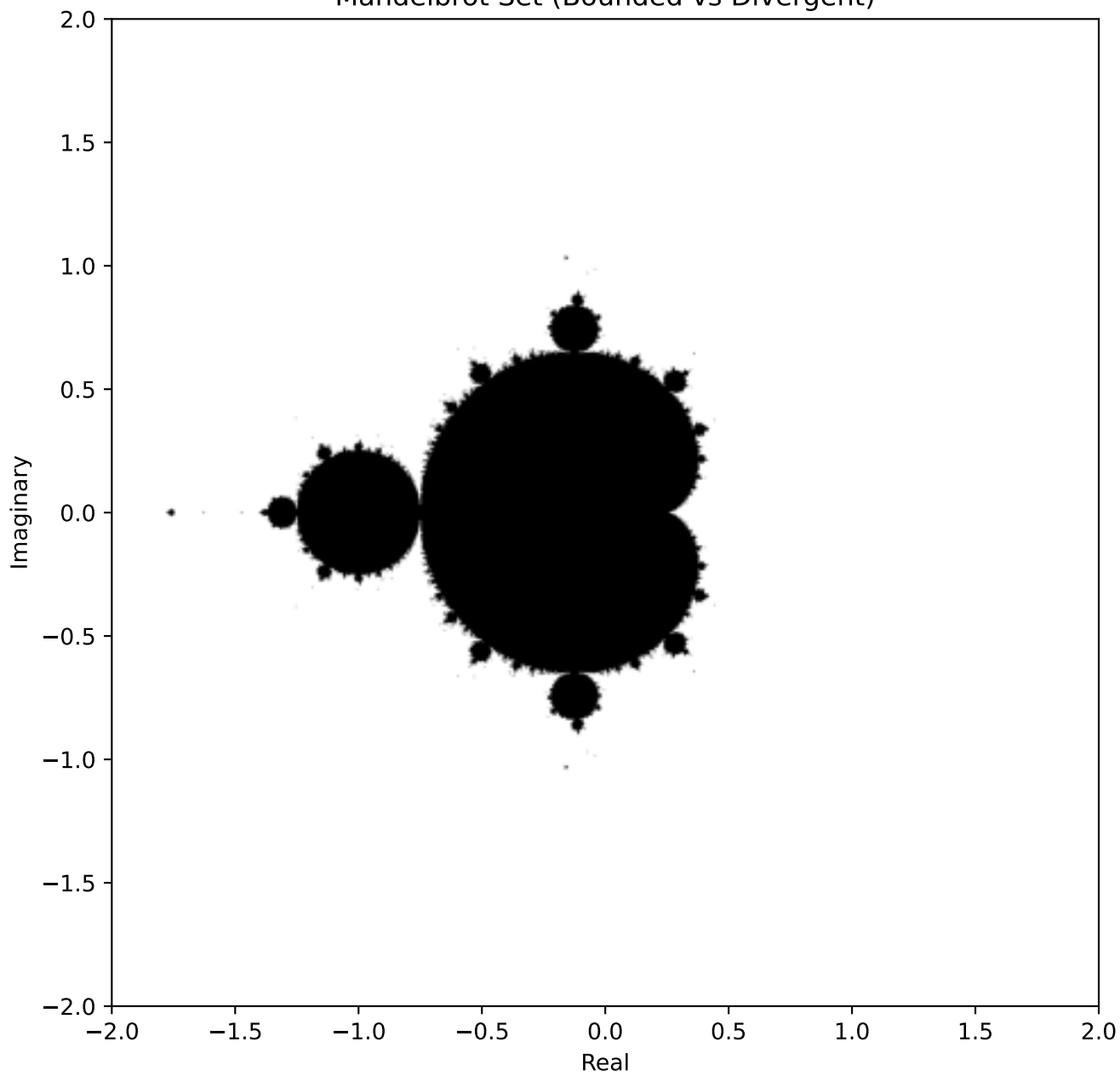
Mandelbrot Set (Bounded vs Divergent)
