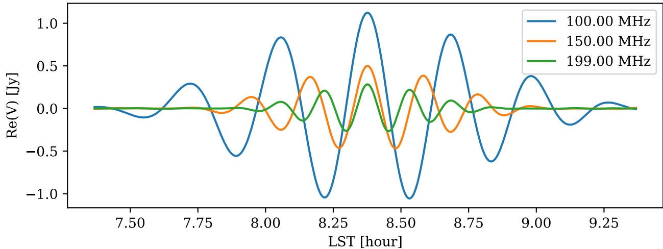
Re(V) Time Series (0,3) | 59.4 m
