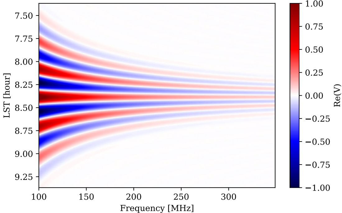
Re(V) Waterfall (1,2)
