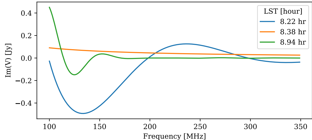
Imaginary Part of Visibility vs Frequency
