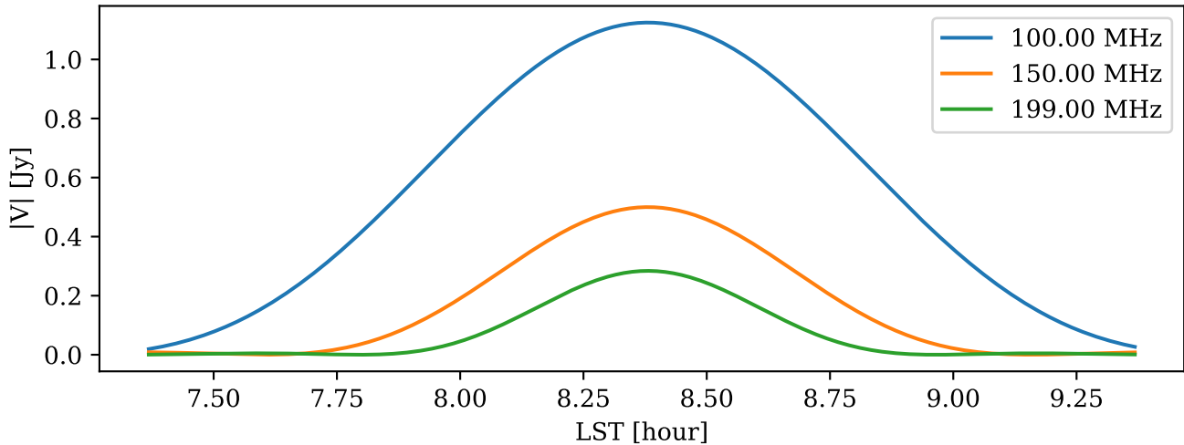
|V| Time Series (0,2) | 42.0 m
