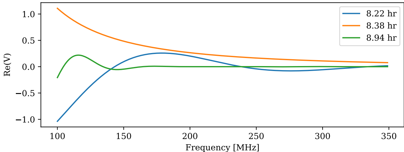
Re(V) Frequency (1,2)
