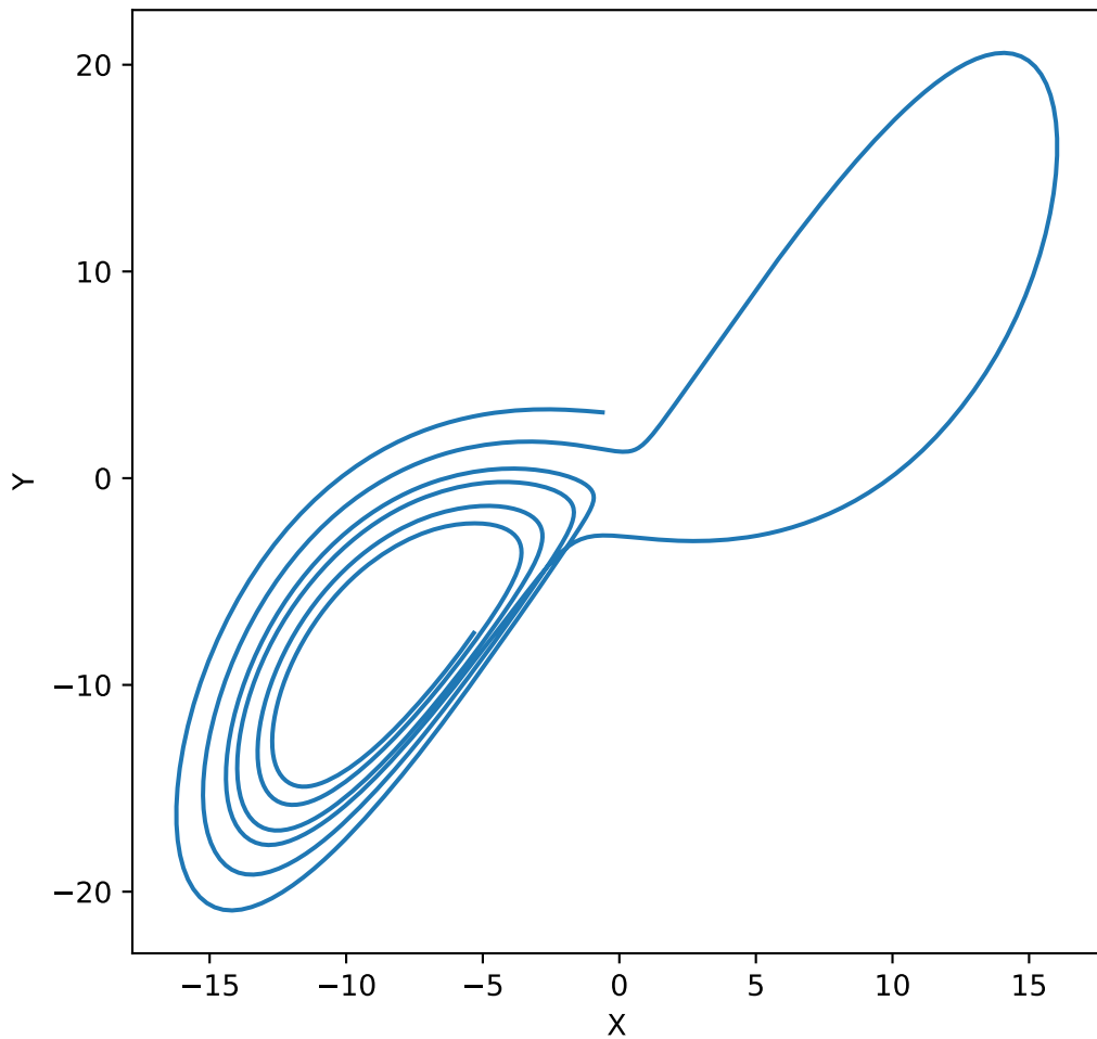
Lorenz Phase Space (X vs Y)
