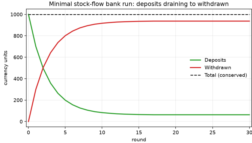
Figure 1: A minimal lethain stock-flow bank run: deposits drain into a withdrawn stock under a confidence-dependent leak, with a small return flow, and the total is conserved throughout. This is the bare ledger underneath the reflexive coupling of §5; the basin-selection dynamics that decide whether the run happens live in Fig. 9, not here. An illustrative stock-flow schematic of the conserved-reallocation skeleton.
