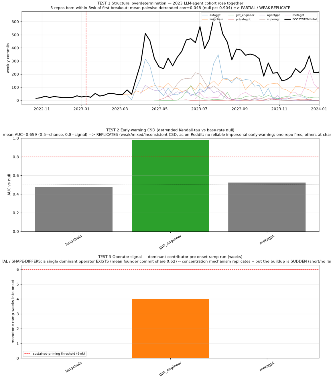
Figure 13: Cross-domain replication on GitHub (2023 agent-framework cohort): the ecosystem commit rise with the eight-week birth cluster (structural priming), the per-repo critical-slowness AUC bars (one repo fires, the rest at chance), and the operator ramp-run weeks (single dominant founder per repo but no sustained pre-cascade ramp). Preliminary, on commit-activity data from the GitHub REST API as an activity proxy for the star-driven attention cascade; n is about three scorable events per test, onsets are heuristic, and the small seven-repo cohort is forced by a 60-requests-per-hour API limit. A preliminary cross-domain probe of reproducibility at small n .
