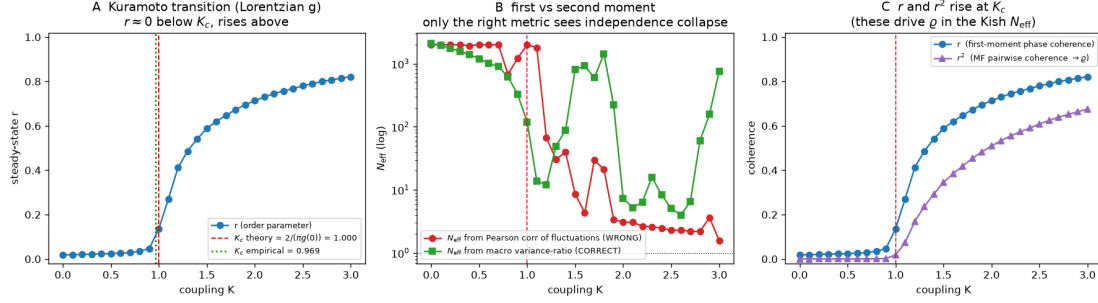
Figure 10: The Kuramoto K_c consistency check (Eq. (7), §6): empirical onset of synchronization in a finite- N simulation ( N = 2000 ) against the theoretical K_c = 2/(\pi g(0)) . The Lorentzian frequency distribution matches to 3.1% and the Gaussian to 27.7%, the latter gap attributable to finite- N and slow convergence near K_c . This is an internal-consistency check of the reused Strogatz result [25] on a controlled synthetic system.
