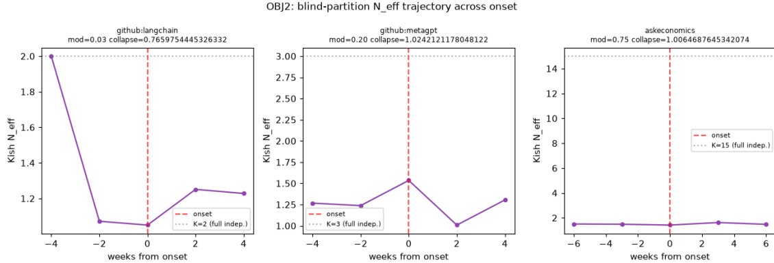
Figure 15: Upgrade 2, blind community detection and Kish N_{\text{eff}} . Blind Louvain on the pre-onset co-participation graph recovers K = 15 to 16 distinct blocks at modularity 0.749 on the 707-node AskEconomics graph, confirming near-decomposability with no outcome selection. The dynamic N_{\text{eff}} collapse is only suggestive: langchain falls 1.54 \rightarrow 1.18 ( n = 1 ), most GitHub repos are born-into-cascade with no pre-onset graph, and the AskEconomics designated onset shows no collapse. Preliminary first-contact result: the structural half is robust, and the collapse dynamic is taken up by the powered two-substrate test of §15.3.
