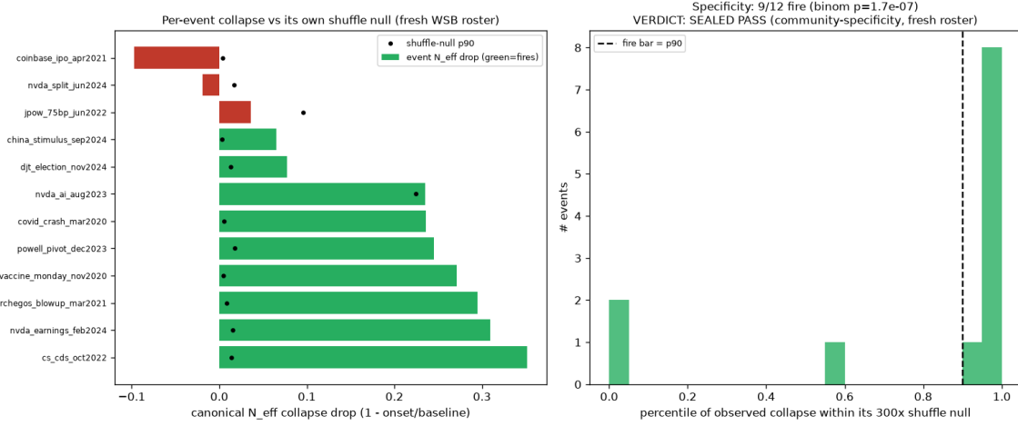
Figure 18: The dynamic N_{\text{eff}} collapse on the endpoint the theory names. r/wallstreetbets, fresh roster of twelve cascades disjoint from every prior run; validation/neff_v4/. Left: per-cascade canonical- N_{\text{eff}} collapse with each cascade's own block-label-shuffle 90th percentile (dots); green bars fire (collapse past the shuffle null), red do not. Right: the observed collapse sits at the very top of its own 300-shuffle distribution for most cascades (median percentile 1.00). Nine of twelve fire, a binomial p = 1.7 \times 10^{-7} . The dots on the left panel also show the substrate's null geometry: ten of the twelve nulls sit below 0.018 while the bars they gate run to 0.35, so on this forum the specificity bar is low in absolute terms. On the two cascades whose null is on the scale of the collapses being scored the endpoint discriminates as designed, one firing at the ninety-first percentile and one correctly silent. The September-2024 case (raw collapse only 0.065 yet above all 300 shuffles, its null's 90th percentile being 0.0028) is the sharpest illustration of why specificity and magnitude are different quantities on this substrate.
