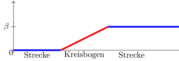
Figure 26.2.: Angular change with blending arc
