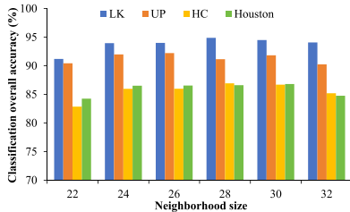
Fig. 6. OA(%) with different neighborhood sizes on four HSI datasets.
