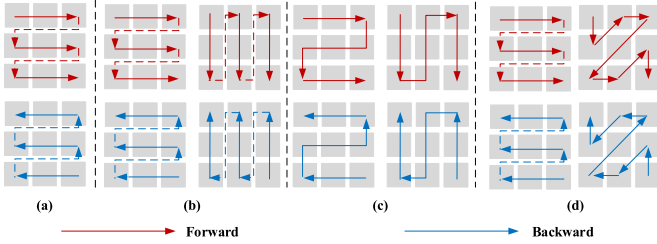
Fig. 3. Illustration of different scanning methods. (a) Horizontal. (b) Horizontal/vertical. (c) Horizontal/vertical zigzag. (d) Horizontal/diagonal zigzag.
