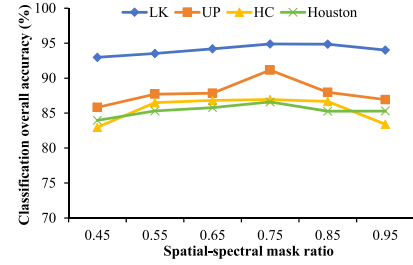
Fig. 5. OA(%) with different spatial-spectral mask ratios on four HSI datasets.
