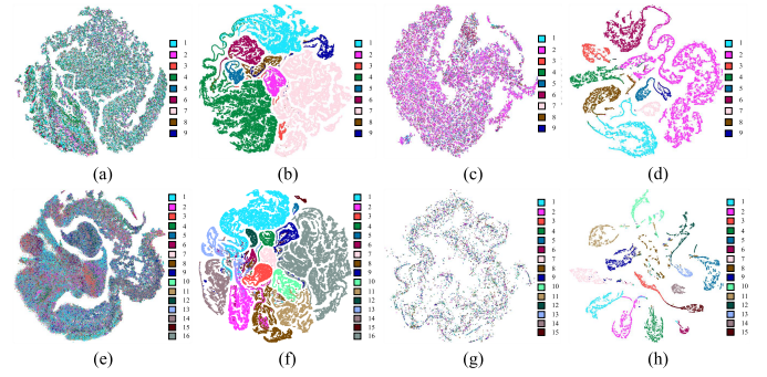
Fig. 11. T-SNE visualization of raw versus SSUpMamba features for (a) and (b) LK, (c) and (d) UP, (e) and (f) HC, and (g) and (h) HU datasets.
