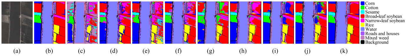
Fig. 7. Classification maps for the WHU-Hi-LongKou dataset. (a) False-color image (29, 19, 9). (b) Ground truth. (c) PCA+SVM. (d) SSTN. (e) MambaHSI. (f) DCFSL. (g) SS-MTr. (h) C-SS-MTr. (i) TCRL. (j) CMLPL. (k) Proposed SSUpMamba.
