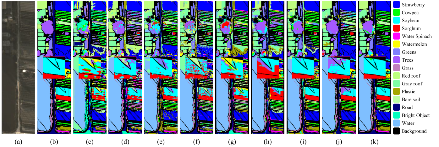
Fig. 9. Classification maps for the WHU-Hi-HanChuan dataset. (a) False-color image (29, 19, 9). (b) Ground truth. (c) PCA+SVM. (d) SSTN. (e) MambaHSI. (f) DCFSL. (g) SS-MTr. (h) C-SS-MTr. (i) TCRL. (j) CMLPL. (k) Proposed SSUpMamba.
