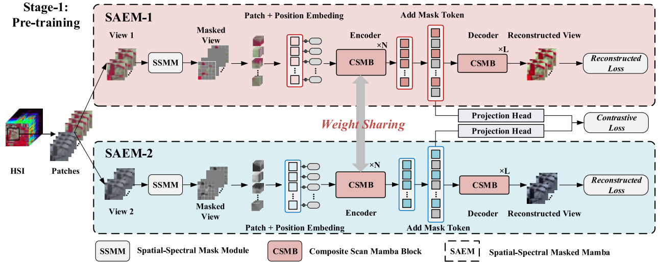
Fig. 1. Overview of the proposed SSUpMamba. Given an HSI, samples are first collected centered around each ground object. The sampled patches are then divided into two groups on average by band, with each group being treated as a view of the HSI. During the self-supervised pretraining phase (Stage-1), these views are fed into two SAEM networks (SAEM-1/2). While architecturally identical, SAEM-1 and SAEM-2 specialize in learning view-specific representations through shared-encoder/independent-decoder configurations.
