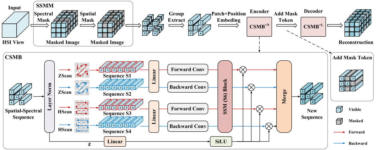
Fig. 4. SAEM and SSMM. Given image blocks from a view, they are cropped according to a specific neighborhood size and then input into SSMM. Subsequently, spectral band masking and spatial masking are applied sequentially based on specific masking rates. The CSMB—the spatial-spectral embedding sequences of HSI—traverse along four different scanning paths, each sequence independently processed by different S6 blocks. Subsequently, the results are merged into a feature map as the ultimate output (cross-merging).
