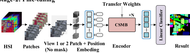
Fig. 2. Fine-tuning stage of the proposed SSUpMamba. After pretraining, the encoding component of SAEM is used as a feature extractor, and a classification head is added to obtain the final results (Stage-2).
