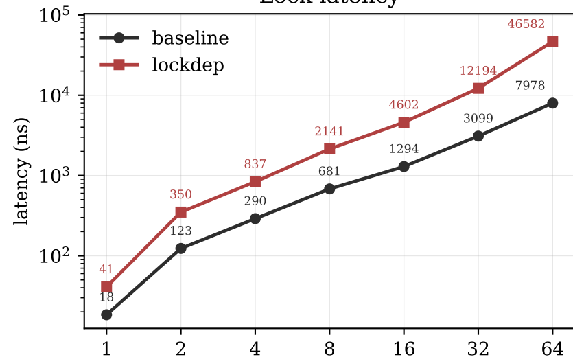
Lockdep added delay
