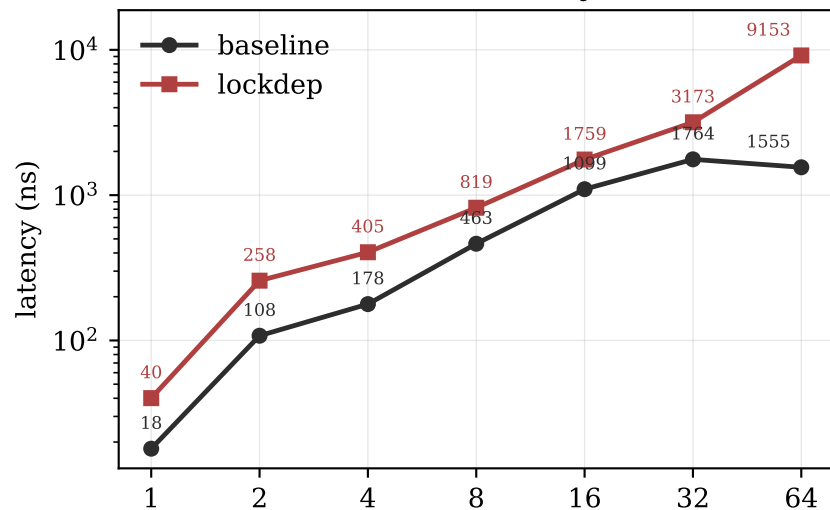
Lock+unlock pair overhead
