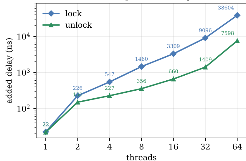
Lockdep added delay
