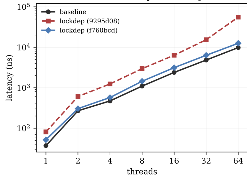
Lock+unlock pair latency
