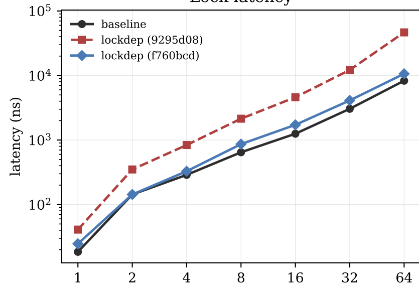
Lock+unlock pair latency
