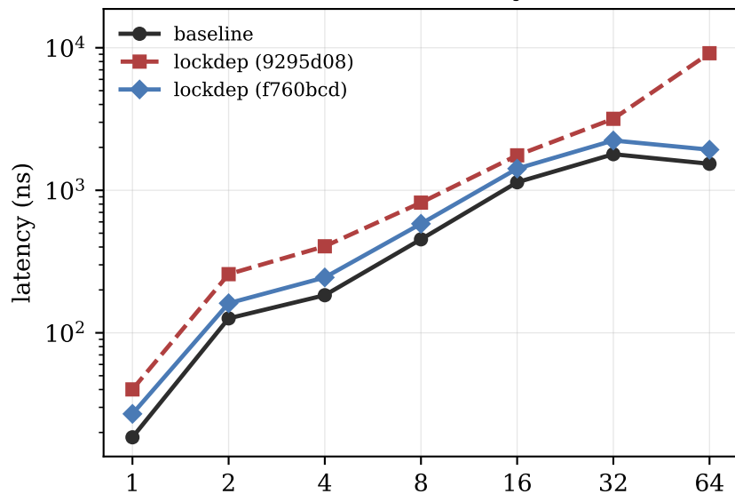
Lock+unlock pair overhead
