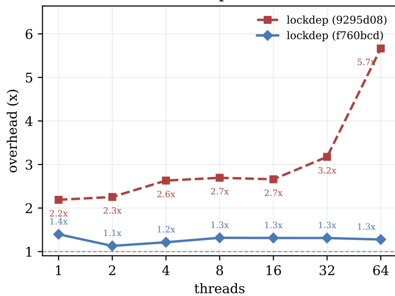
Lock+unlock pair overhead
