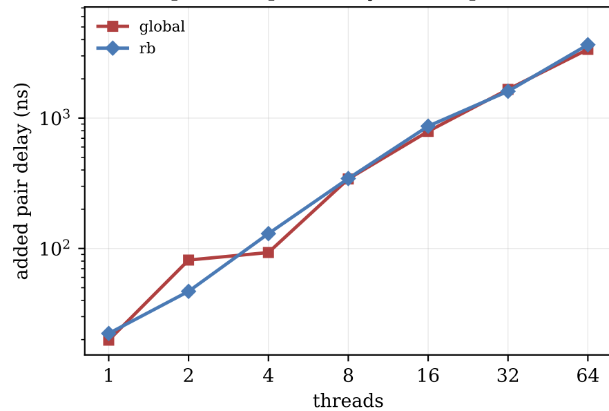
Lockdep added pair delay (lockdep - baseline)
