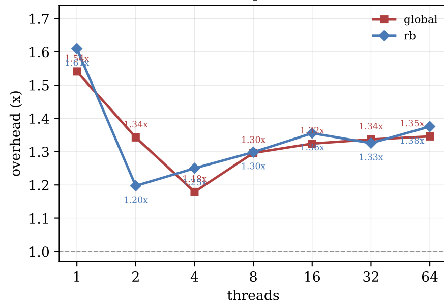
Lock+unlock pair overhead
