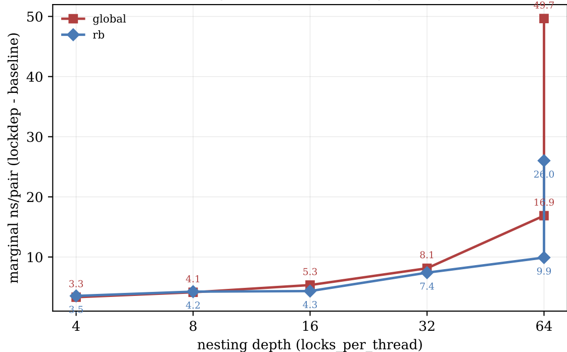
Marginal cost vs nesting depth
