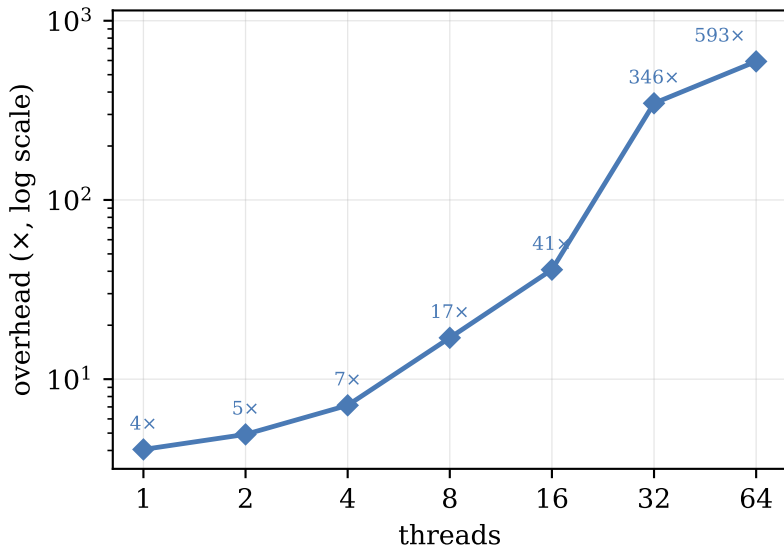
Low contention — overhead factor
