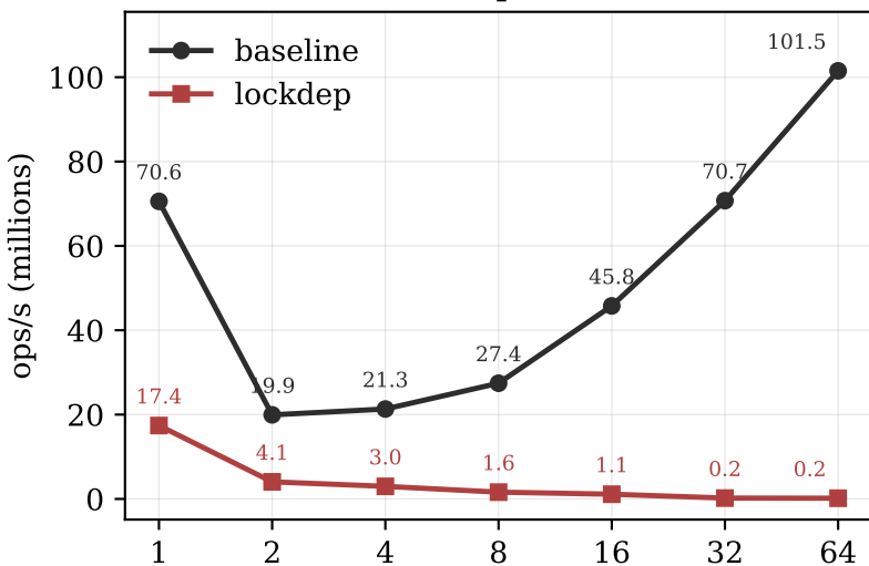
Low contention (per-thread locks)
