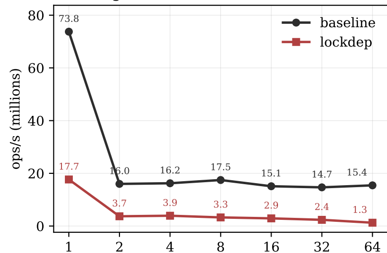
High contention (1 shared lock)
