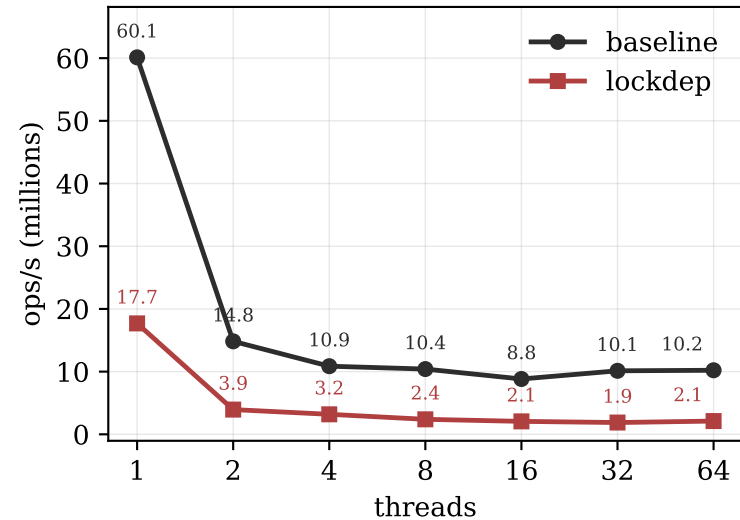
Throughput
