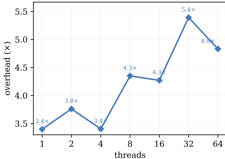
Overhead factor
