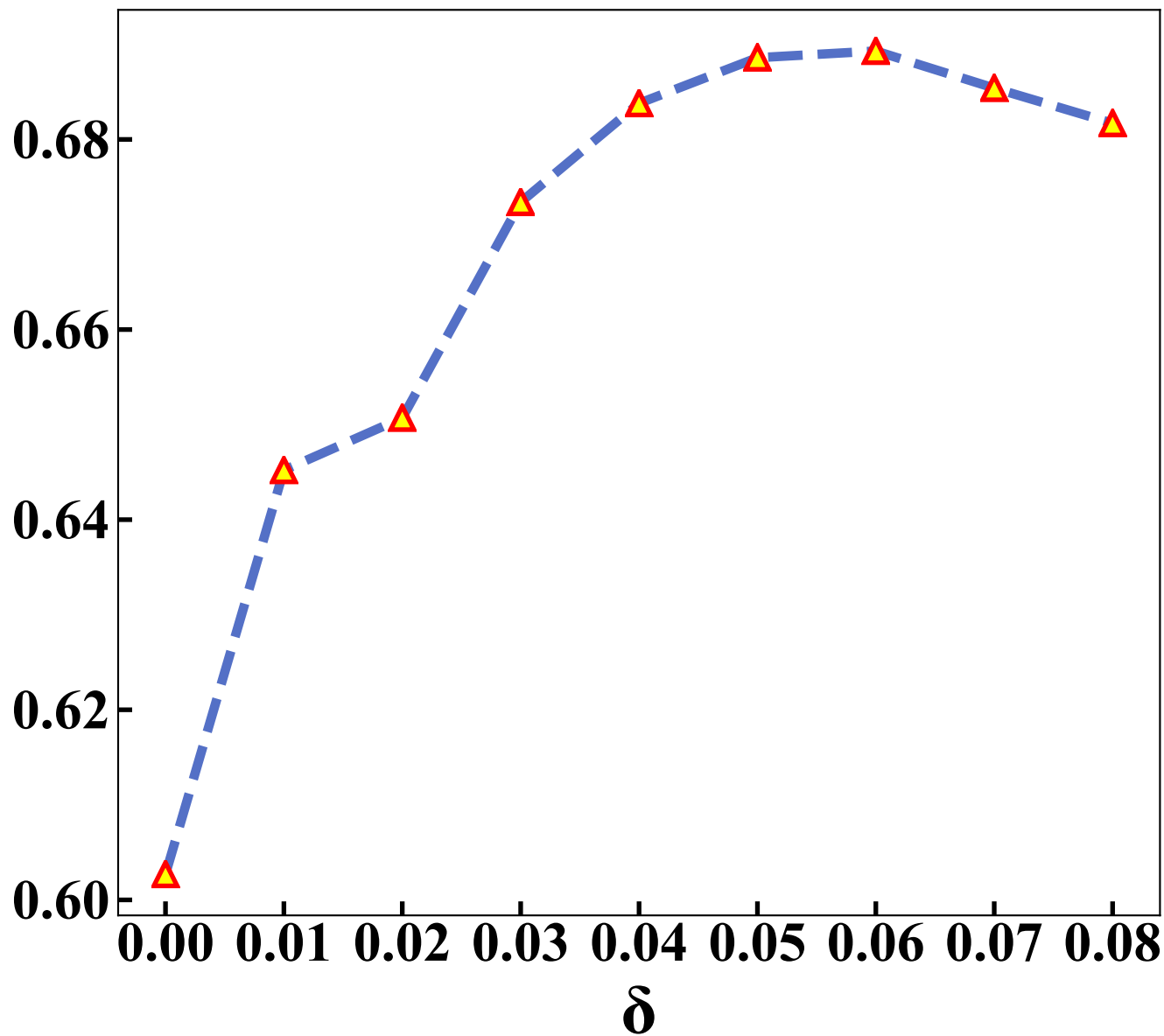
F1-score
