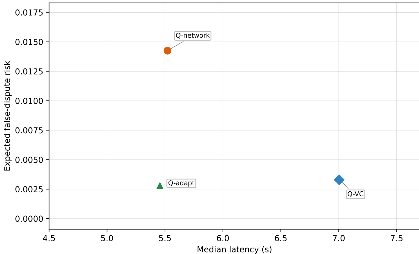
A3 queue-aware frontier at queued-8, alpha=0.10
