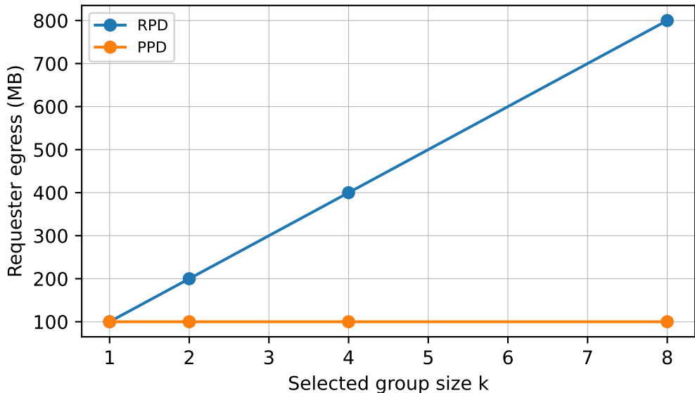
Requester egress under placement-defined disclosure
