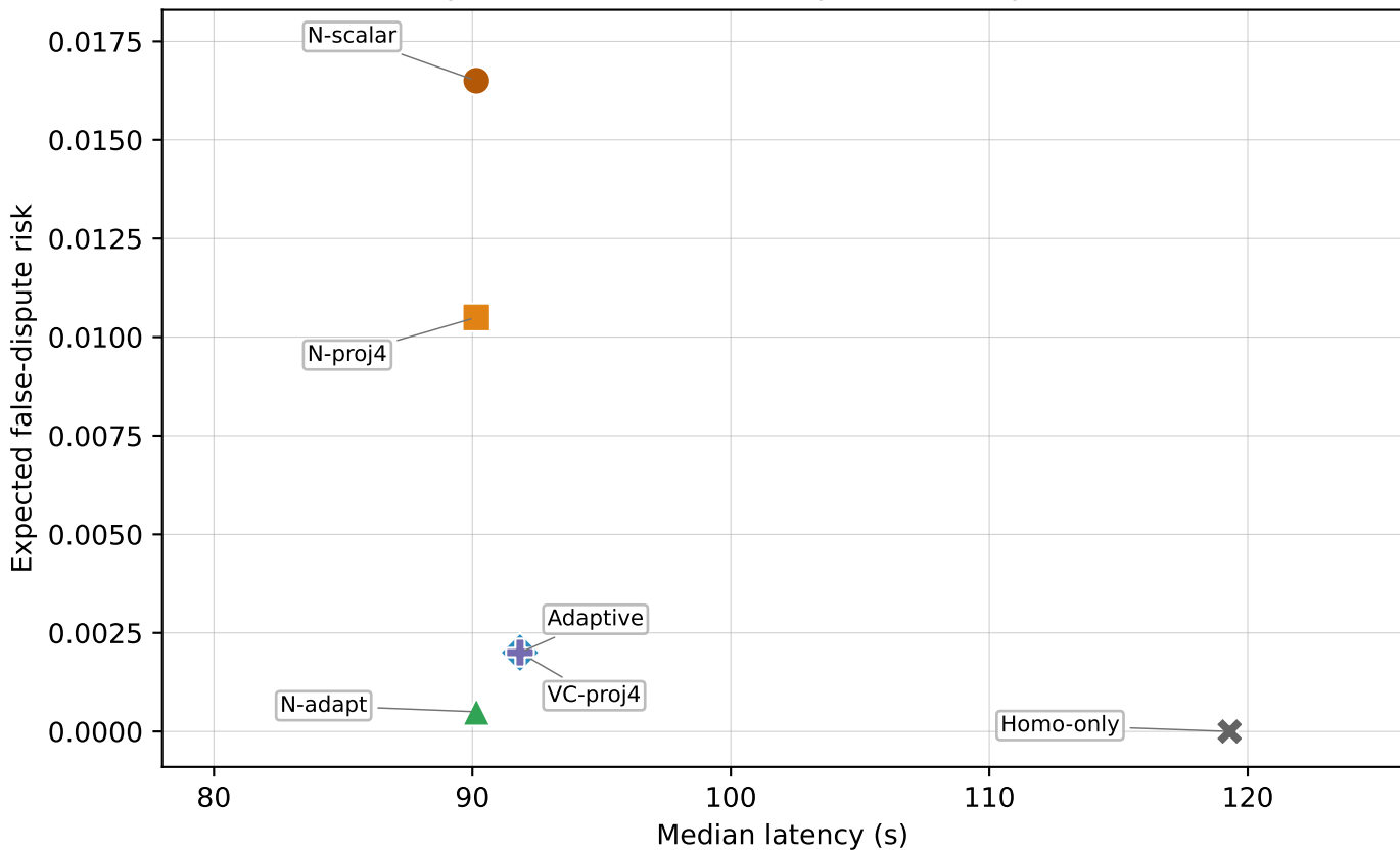
A1 placement frontier at queued-8, alpha=0.10
